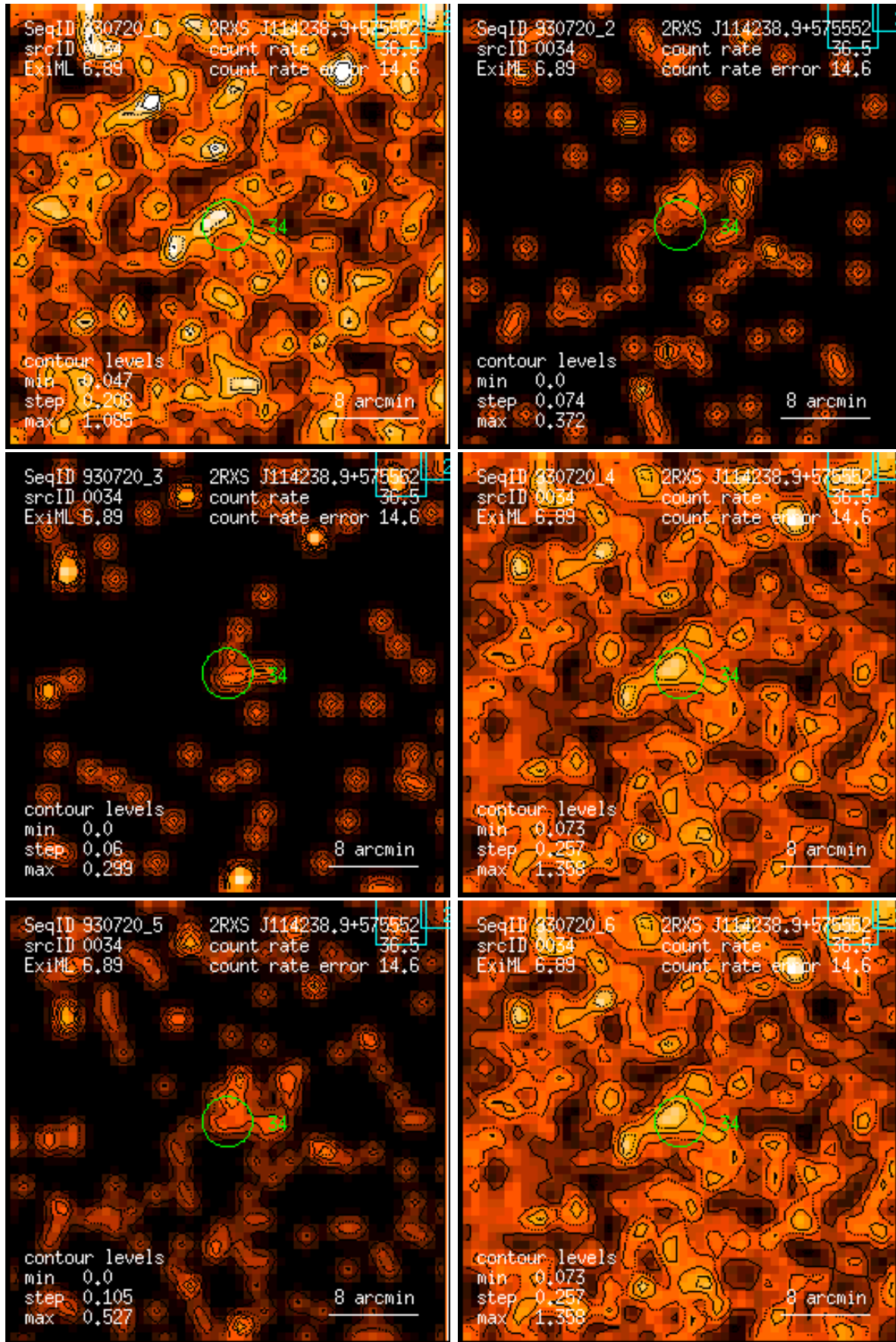
Figure 34: RASS 930720: detection 0034: band rate images, Gaussian filter: (1) PSPC channels 11 – 41, (2) 52 – 90, (3) 91 – 201, (4) 11 – 235, (5) 52 – 201, (6) 11 – 201. Broad band rates in counts/ks. Band rate contour levels in counts/ks/arcmin 2 .
