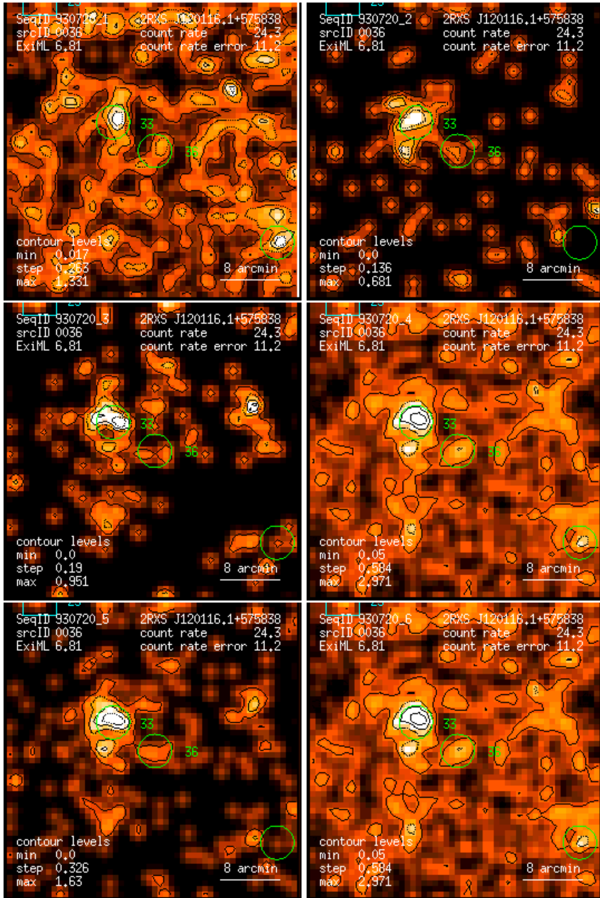
Figure 36: RASS 930720: detection 0036: band rate images, Gaussian filter: (1) PSPC channels 11 – 41, (2) 52 – 90, (3) 91 – 201, (4) 11 – 235, (5) 52 – 201, (6) 11 – 201. Broad band rates in counts/ks. Band rate contour levels in counts/ks/arcmin 2 .
