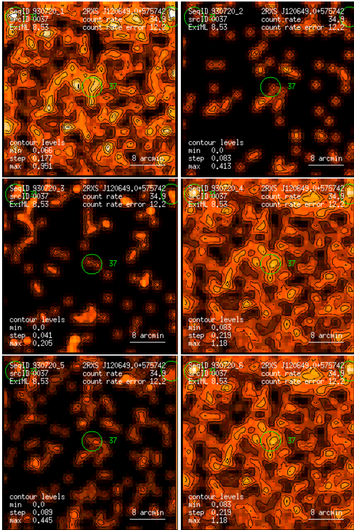
Figure 37: RASS 930720: detection 0037: band rate images, Gaussian filter: (1) PSPC channels 11 – 41, (2) 52 – 90, (3) 91 – 201, (4) 11 – 235, (5) 52 – 201, (6) 11 – 201. Broad band rates in counts/ks. Band rate contour levels in counts/ks/arcmin 2 .
