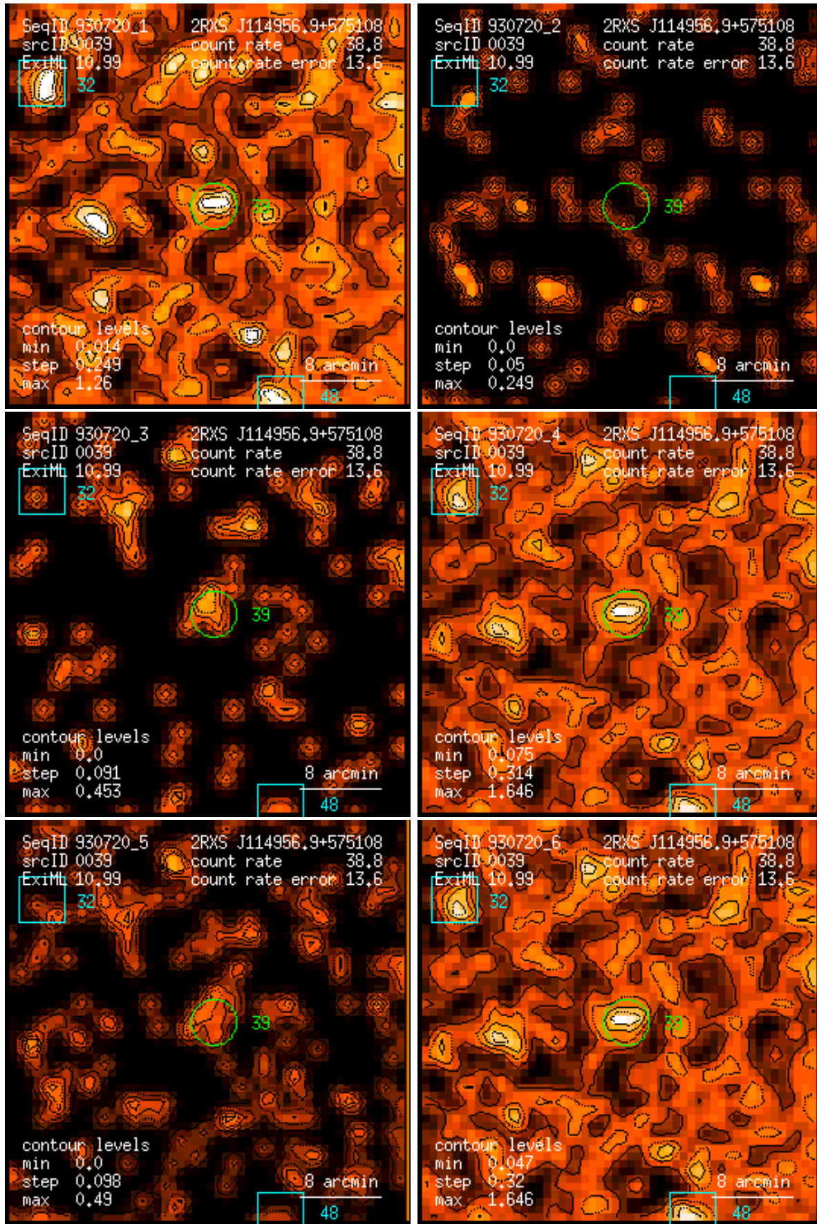
Figure 39: RASS 930720: detection 0039: band rate images, Gaussian filter: (1) PSPC channels 11 – 41, (2) 52 – 90, (3) 91 – 201, (4) 11 – 235, (5) 52 – 201, (6) 11 – 201. Broad band rates in counts/ks. Band rate contour levels in counts/ks/arcmin 2 .
