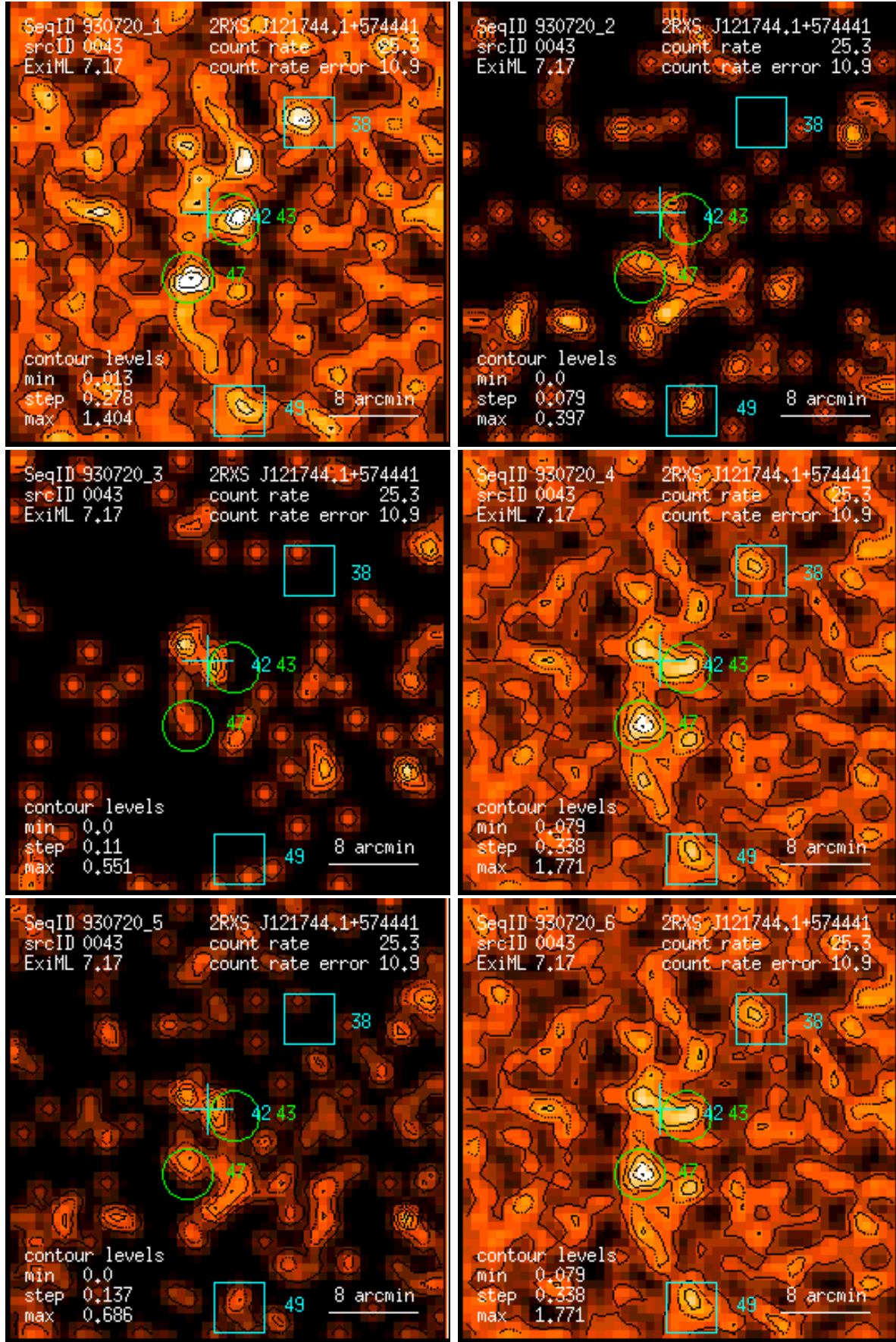
Figure 43: RASS 930720: detection 0043: band rate images, Gaussian filter: (1) PSPC channels 11 – 41, (2) 52 – 90, (3) 91 – 201, (4) 11 – 235, (5) 52 – 201, (6) 11 – 201. Broad band rates in counts/ks. Band rate contour levels in counts/ks/arcmin 2 .
