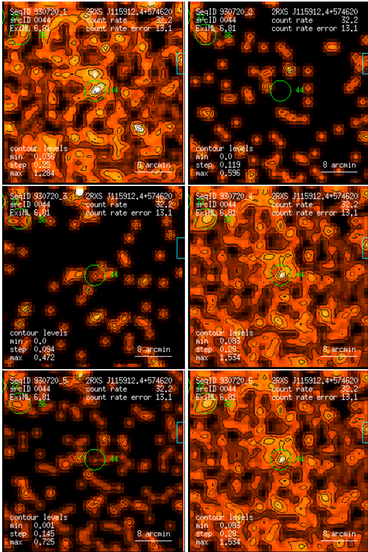
Figure 44: RASS 930720: detection 0044: band rate images, Gaussian filter: (1) PSPC channels 11 – 41, (2) 52 – 90, (3) 91 – 201, (4) 11 – 235, (5) 52 – 201, (6) 11 – 201. Broad band rates in counts/ks. Band rate contour levels in counts/ks/arcmin 2 .
