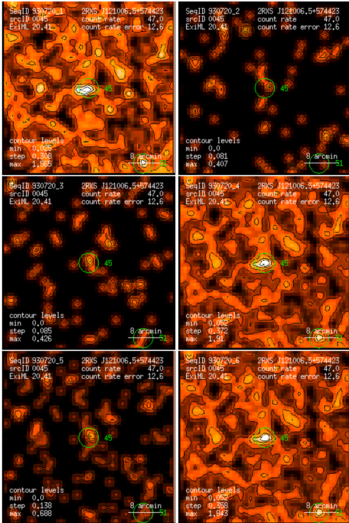
Figure 45: RASS 930720: detection 0045: band rate images, Gaussian filter: (1) PSPC channels 11 – 41, (2) 52 – 90, (3) 91 – 201, (4) 11 – 235, (5) 52 – 201, (6) 11 – 201. Broad band rates in counts/ks. Band rate contour levels in counts/ks/arcmin 2 .
