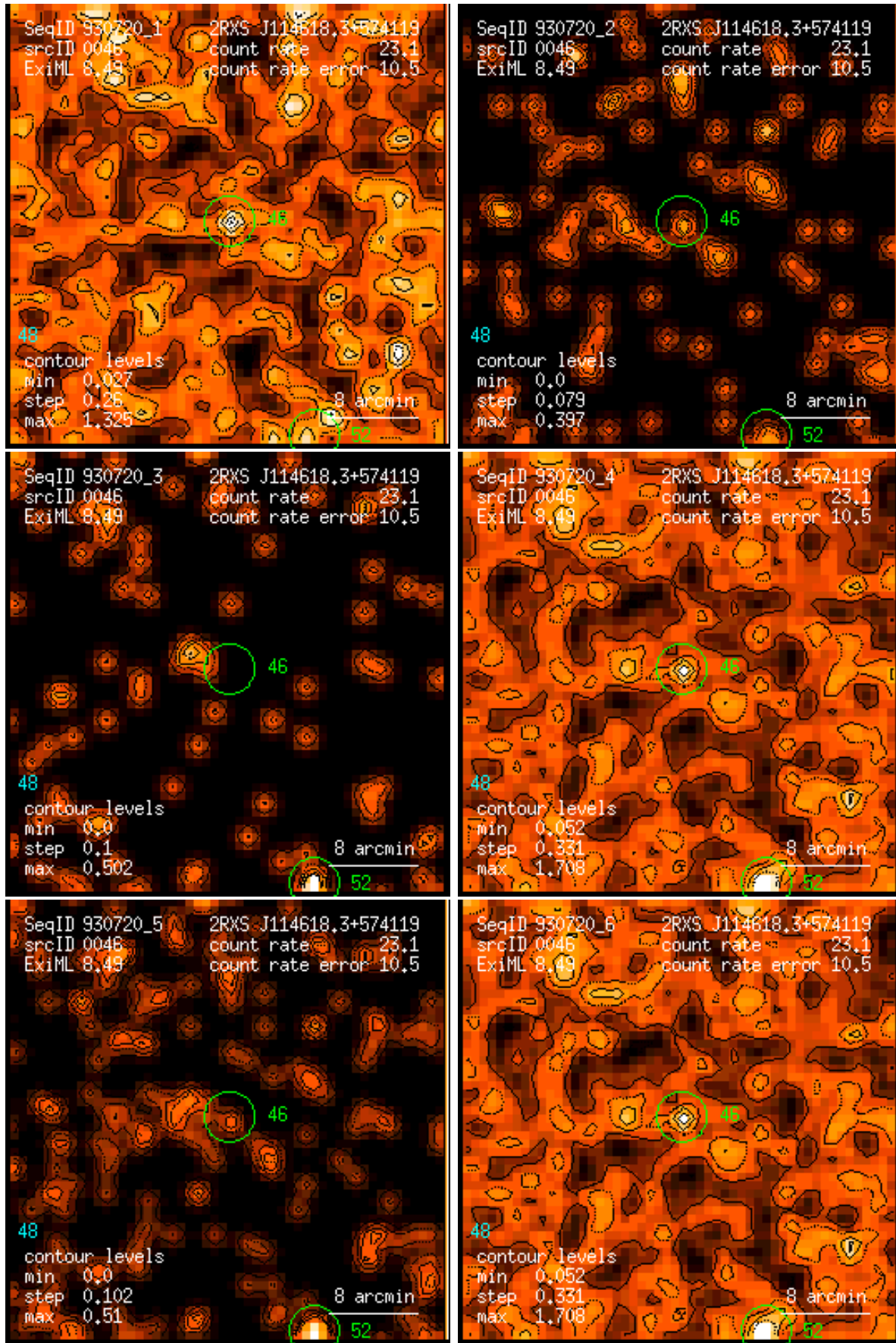
Figure 46: RASS 930720: detection 0046: band rate images, Gaussian filter: (1) PSPC channels 11 – 41, (2) 52 – 90, (3) 91 – 201, (4) 11 – 235, (5) 52 – 201, (6) 11 – 201. Broad band rates in counts/ks. Band rate contour levels in counts/ks/arcmin 2 .
