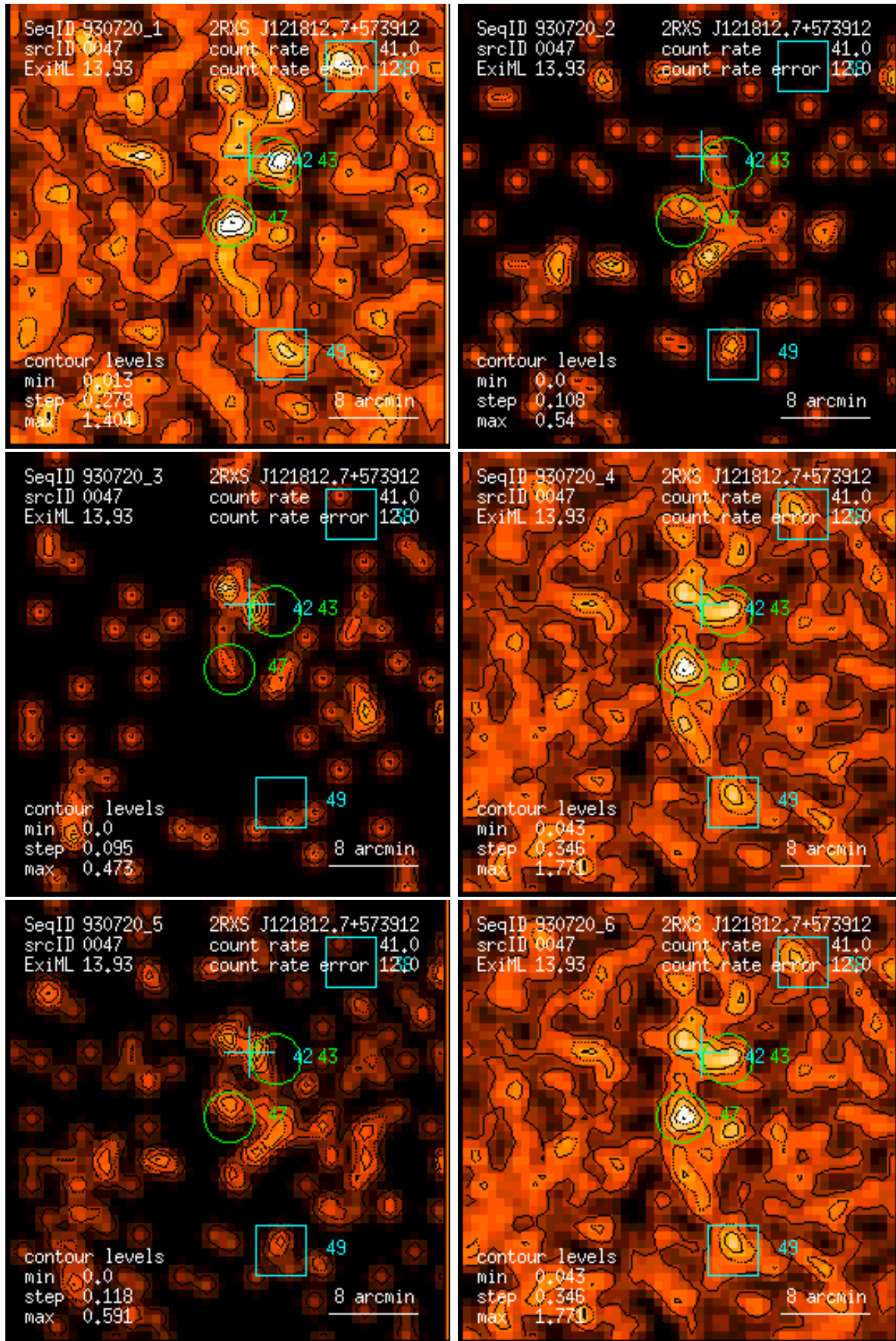
Figure 47: RASS 930720: detection 0047: band rate images, Gaussian filter: (1) PSPC channels 11 – 41, (2) 52 – 90, (3) 91 – 201, (4) 11 – 235, (5) 52 – 201, (6) 11 – 201. Broad band rates in counts/ks. Band rate contour levels in counts/ks/arcmin 2 .
