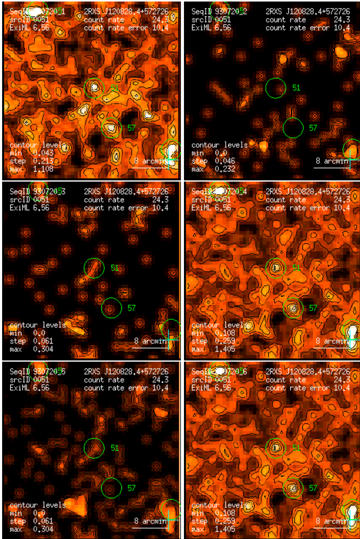
Figure 51: RASS 930720: detection 0051: band rate images, Gaussian filter: (1) PSPC channels 11 – 41, (2) 52 – 90, (3) 91 – 201, (4) 11 – 235, (5) 52 – 201, (6) 11 – 201. Broad band rates in counts/ks. Band rate contour levels in counts/ks/arcmin 2 .
