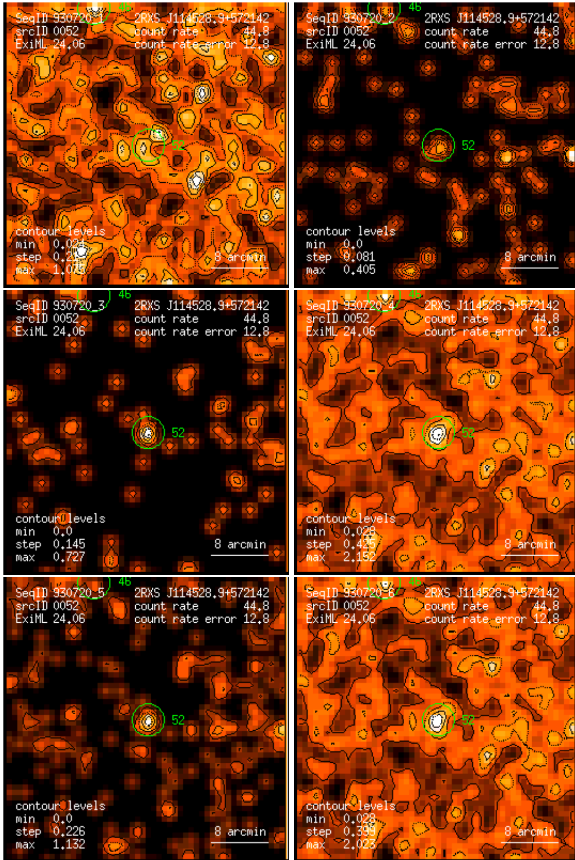
Figure 52: RASS 930720: detection 0052: band rate images, Gaussian filter: (1) PSPC channels 11 – 41, (2) 52 – 90, (3) 91 – 201, (4) 11 – 235, (5) 52 – 201, (6) 11 – 201. Broad band rates in counts/ks. Band rate contour levels in counts/ks/arcmin 2 .
