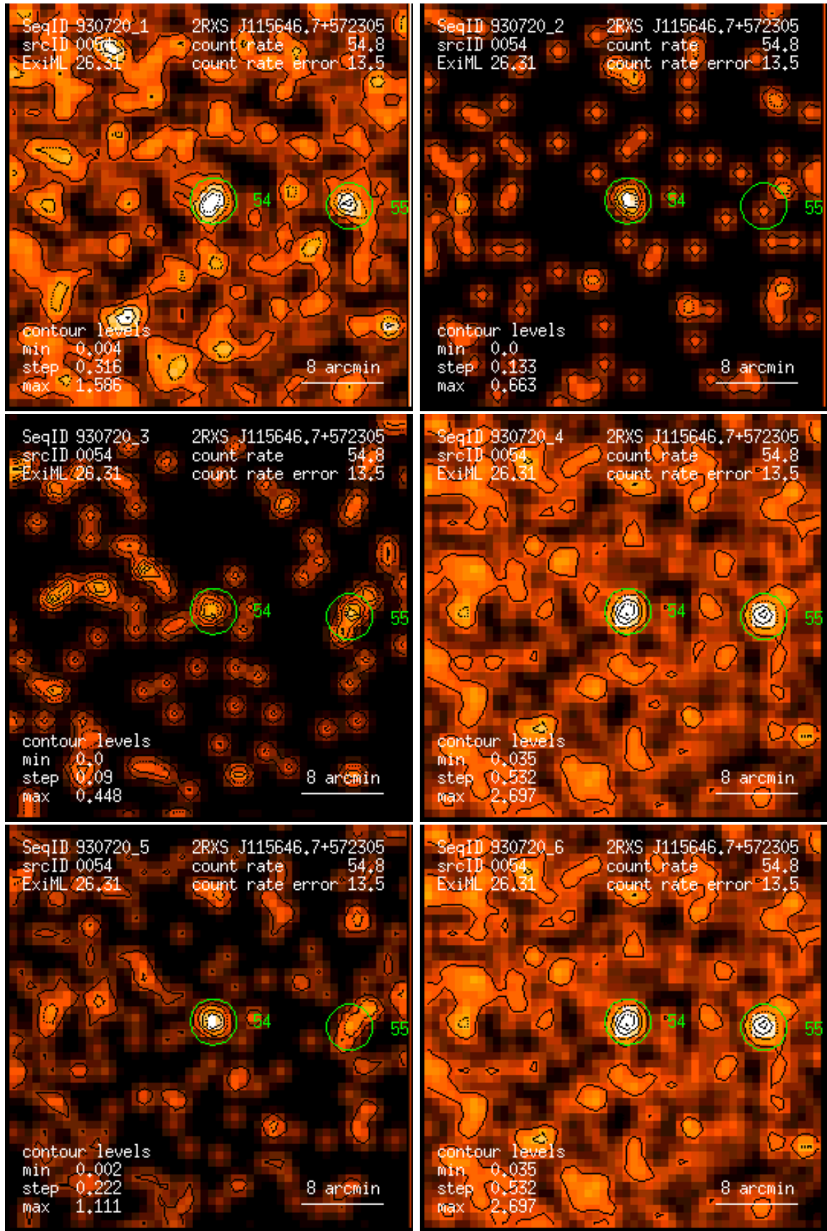
Figure 54: RASS 930720: detection 0054: band rate images, Gaussian filter: (1) PSPC channels 11 – 41, (2) 52 – 90, (3) 91 – 201, (4) 11 – 235, (5) 52 – 201, (6) 11 – 201. Broad band rates in counts/ks. Band rate contour levels in counts/ks/arcmin 2 .
