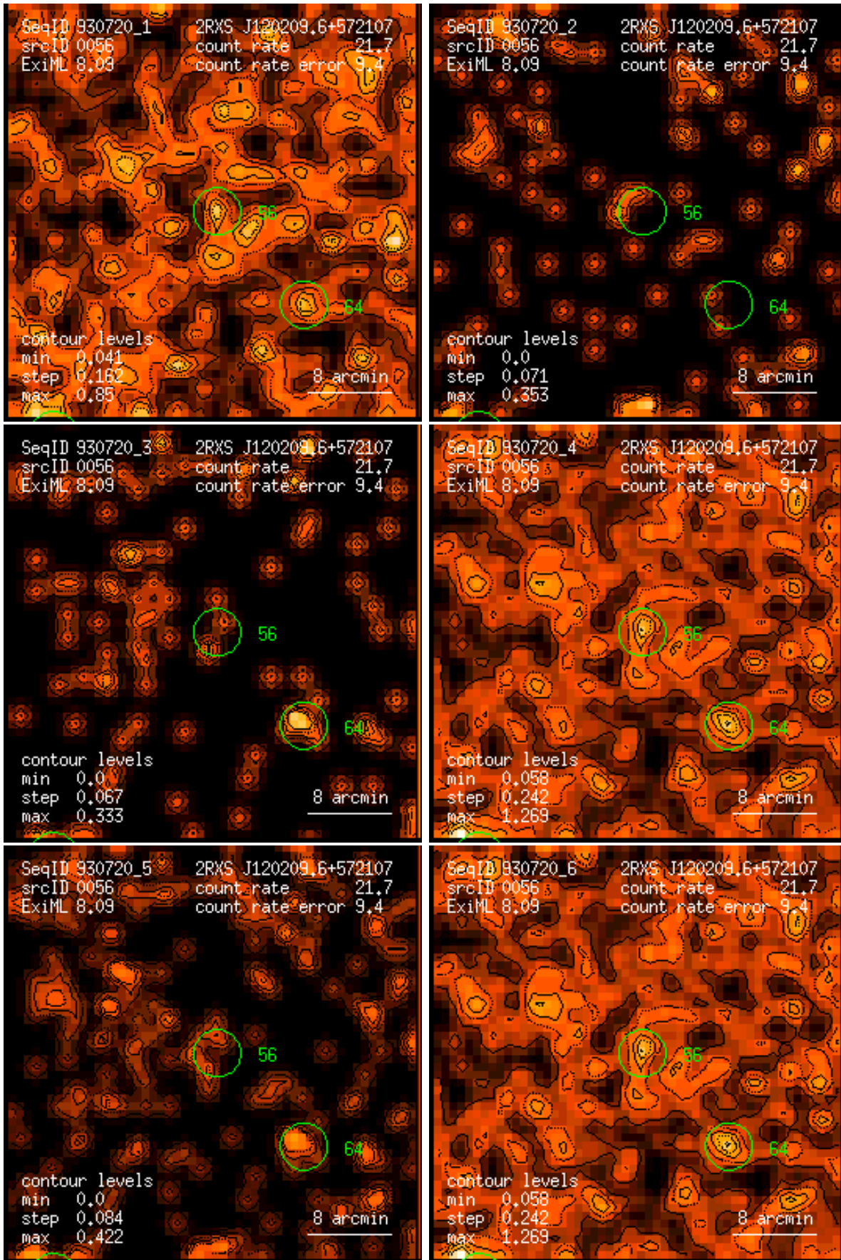
Figure 56: RASS 930720: detection 0056: band rate images, Gaussian filter: (1) PSPC channels 11 – 41, (2) 52 – 90, (3) 91 – 201, (4) 11 – 235, (5) 52 – 201, (6) 11 – 201. Broad band rates in counts/ks. Band rate contour levels in counts/ks/arcmin 2 .
