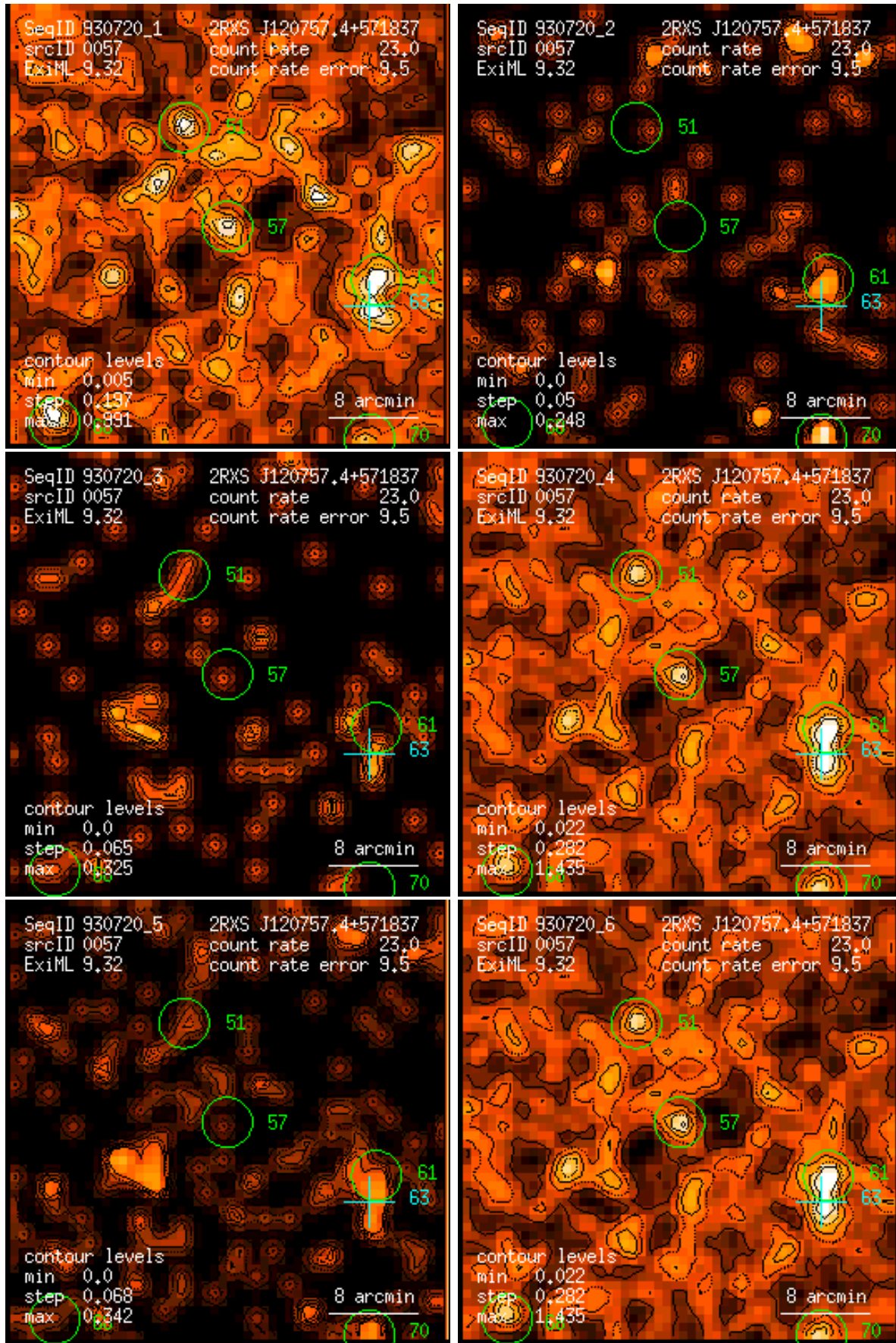
Figure 57: RASS 930720: detection 0057: band rate images, Gaussian filter: (1) PSPC channels 11 – 41, (2) 52 – 90, (3) 91 – 201, (4) 11 – 235, (5) 52 – 201, (6) 11 – 201. Broad band rates in counts/ks. Band rate contour levels in counts/ks/arcmin 2 .
