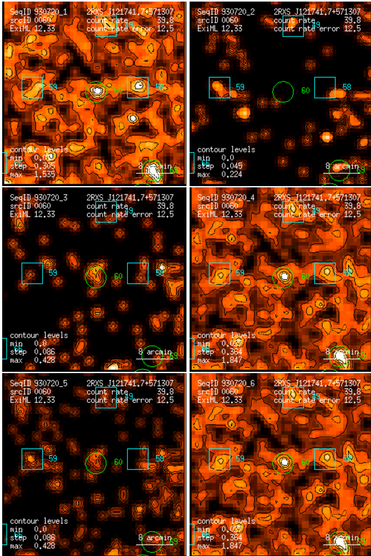
Figure 60: RASS 930720: detection 0060: band rate images, Gaussian filter: (1) PSPC channels 11 – 41, (2) 52 – 90, (3) 91 – 201, (4) 11 – 235, (5) 52 – 201, (6) 11 – 201. Broad band rates in counts/ks. Band rate contour levels in counts/ks/arcmin 2 .
