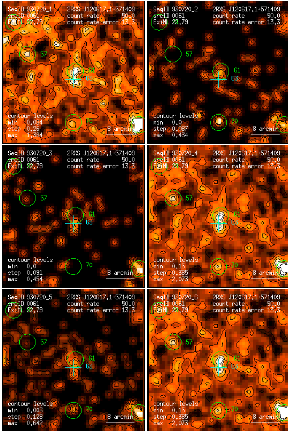
Figure 61: RASS 930720: detection 0061: band rate images, Gaussian filter: (1) PSPC channels 11 – 41, (2) 52 – 90, (3) 91 – 201, (4) 11 – 235, (5) 52 – 201, (6) 11 – 201. Broad band rates in counts/ks. Band rate contour levels in counts/ks/arcmin 2 .
