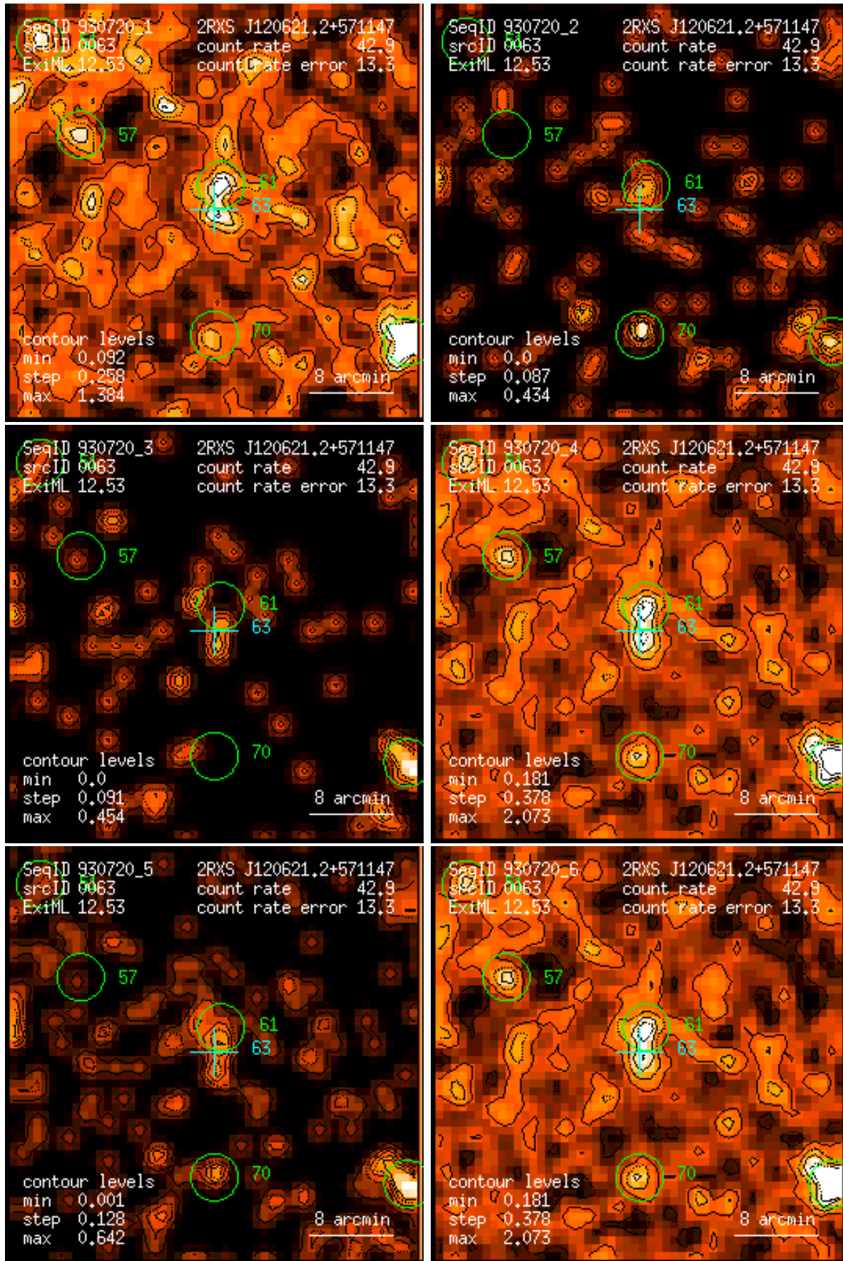
Figure 63: RASS 930720: detection 0063: band rate images, Gaussian filter: (1) PSPC channels 11 – 41, (2) 52 – 90, (3) 91 – 201, (4) 11 – 235, (5) 52 – 201, (6) 11 – 201. Broad band rates in counts/ks. Band rate contour levels in counts/ks/arcmin 2 .
