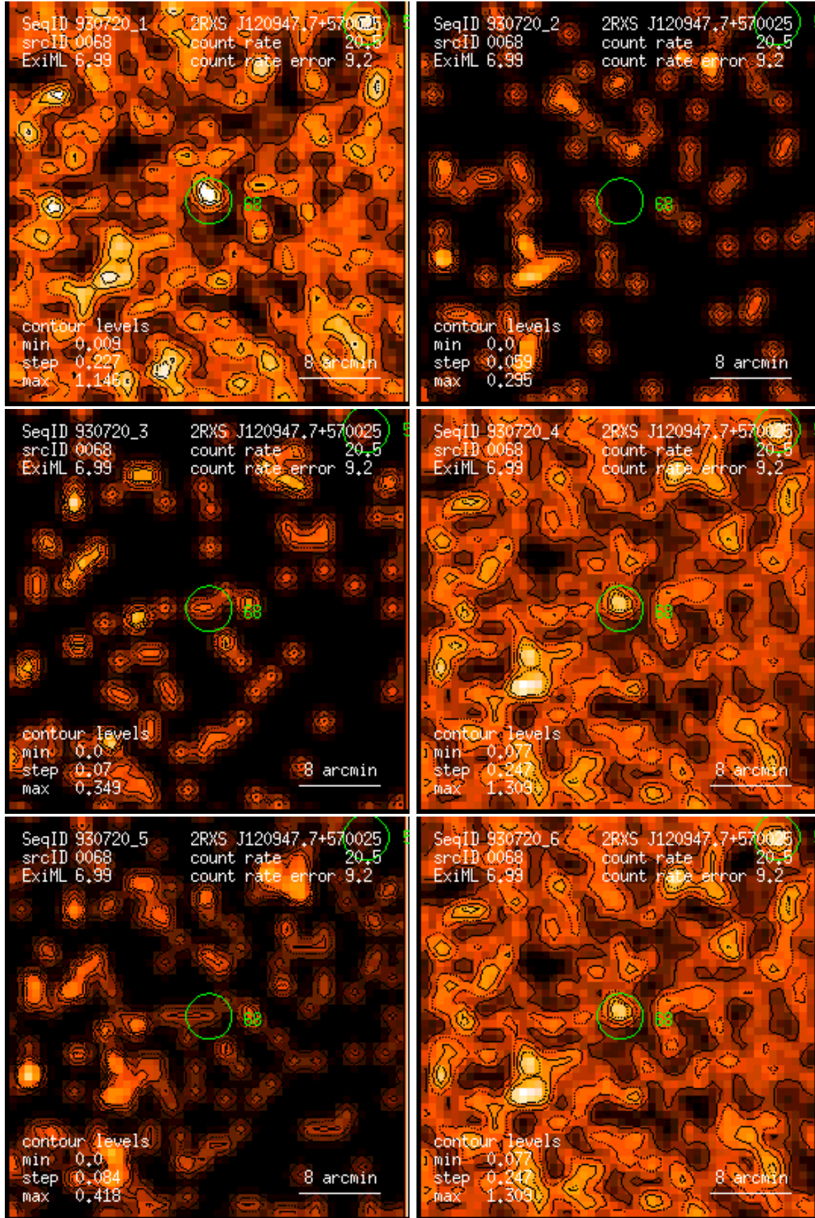
Figure 68: RASS 930720: detection 0068: band rate images, Gaussian filter: (1) PSPC channels 11 – 41, (2) 52 – 90, (3) 91 – 201, (4) 11 – 235, (5) 52 – 201, (6) 11 – 201. Broad band rates in counts/ks. Band rate contour levels in counts/ks/arcmin 2 .
