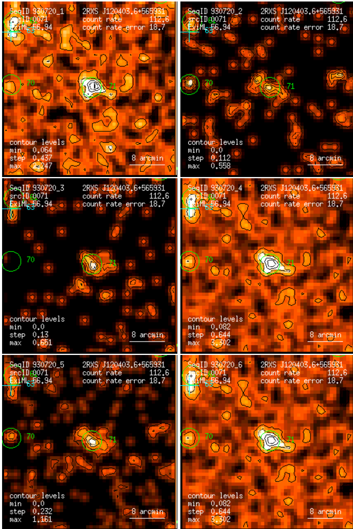
Figure 71: RASS 930720: detection 0071: band rate images, Gaussian filter: (1) PSPC channels 11 – 41, (2) 52 – 90, (3) 91 – 201, (4) 11 – 235, (5) 52 – 201, (6) 11 – 201. Broad band rates in counts/ks. Band rate contour levels in counts/ks/arcmin 2 .
