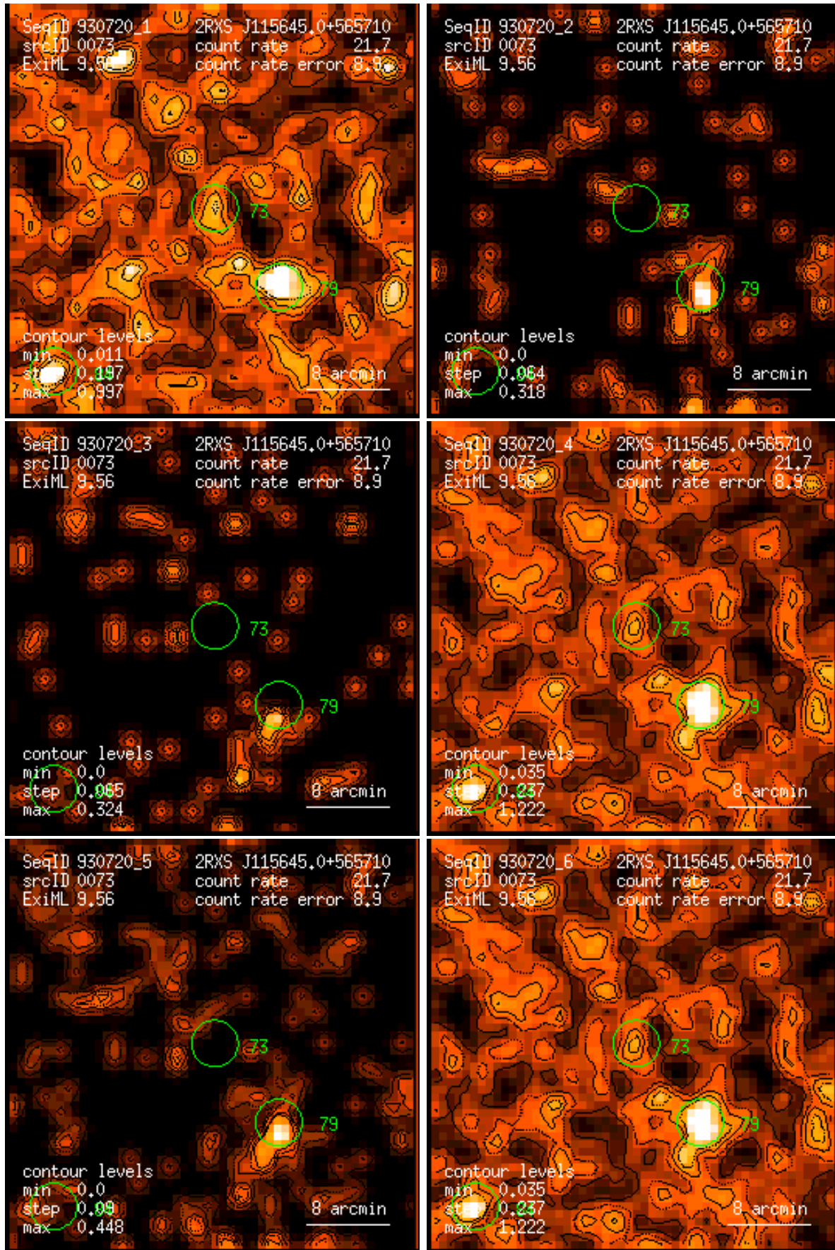
Figure 73: RASS 930720: detection 0073: band rate images, Gaussian filter: (1) PSPC channels 11 – 41, (2) 52 – 90, (3) 91 – 201, (4) 11 – 235, (5) 52 – 201, (6) 11 – 201. Broad band rates in counts/ks. Band rate contour levels in counts/ks/arcmin 2 .
