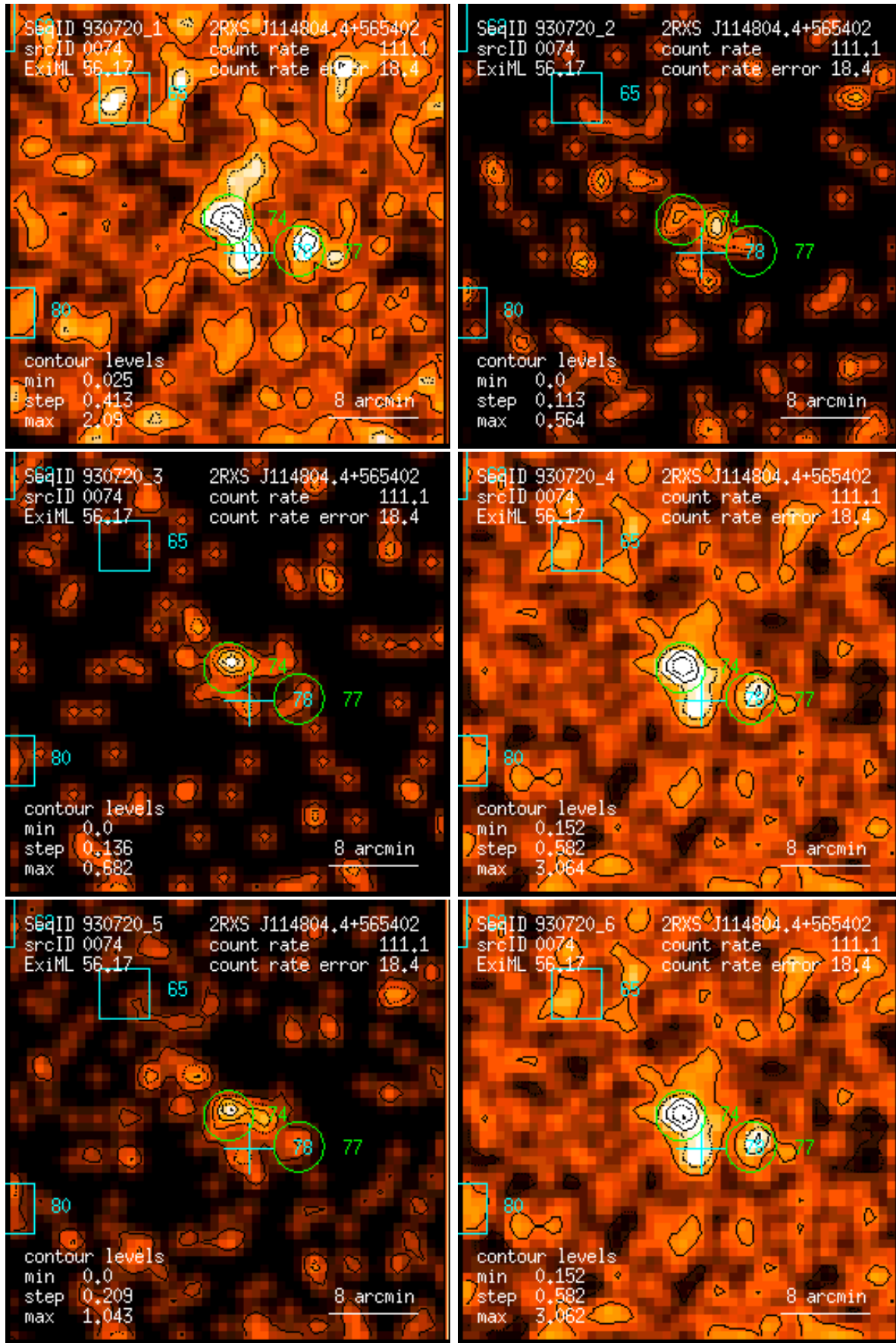
Figure 74: RASS 930720: detection 0074: band rate images, Gaussian filter: (1) PSPC channels 11 – 41, (2) 52 – 90, (3) 91 – 201, (4) 11 – 235, (5) 52 – 201, (6) 11 – 201. Broad band rates in counts/ks. Band rate contour levels in counts/ks/arcmin 2 .
