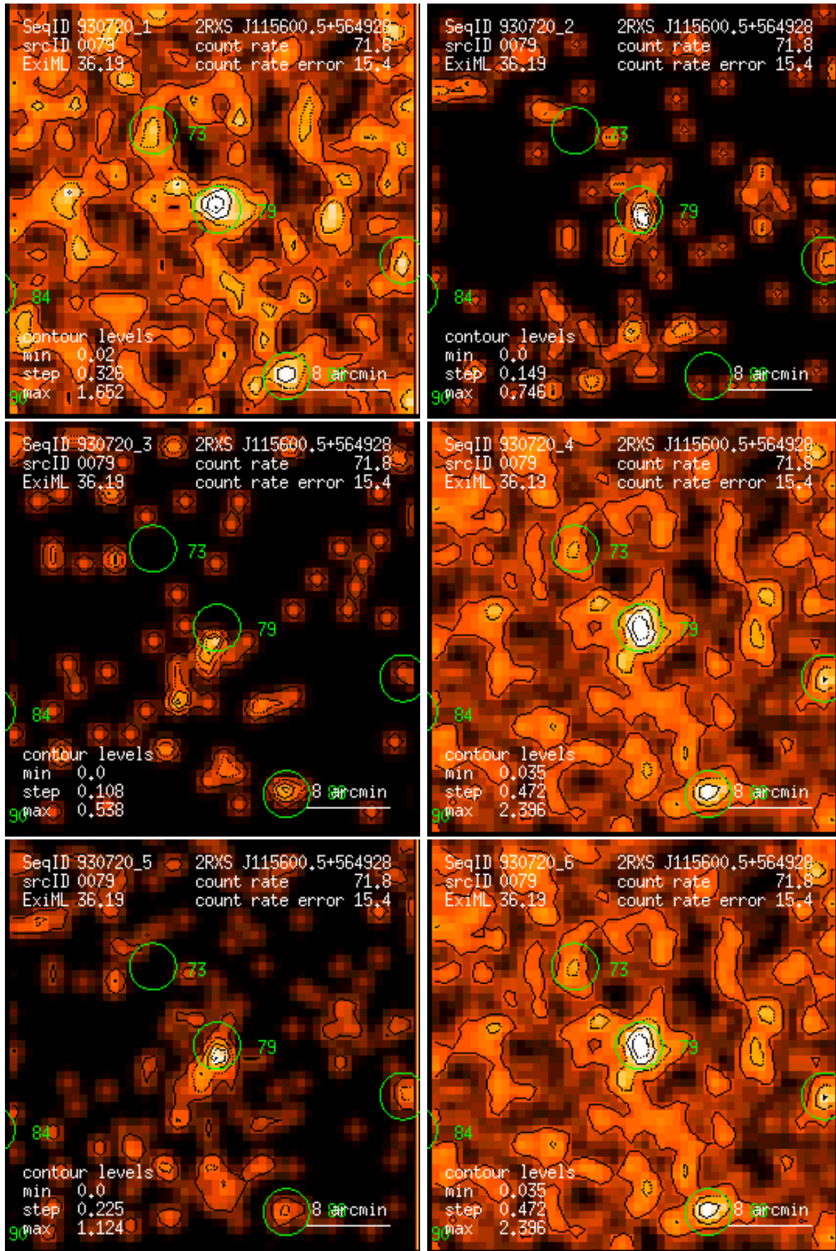
Figure 79: RASS 930720: detection 0079: band rate images, Gaussian filter: (1) PSPC channels 11 – 41, (2) 52 – 90, (3) 91 – 201, (4) 11 – 235, (5) 52 – 201, (6) 11 – 201. Broad band rates in counts/ks. Band rate contour levels in counts/ks/arcmin 2 .
