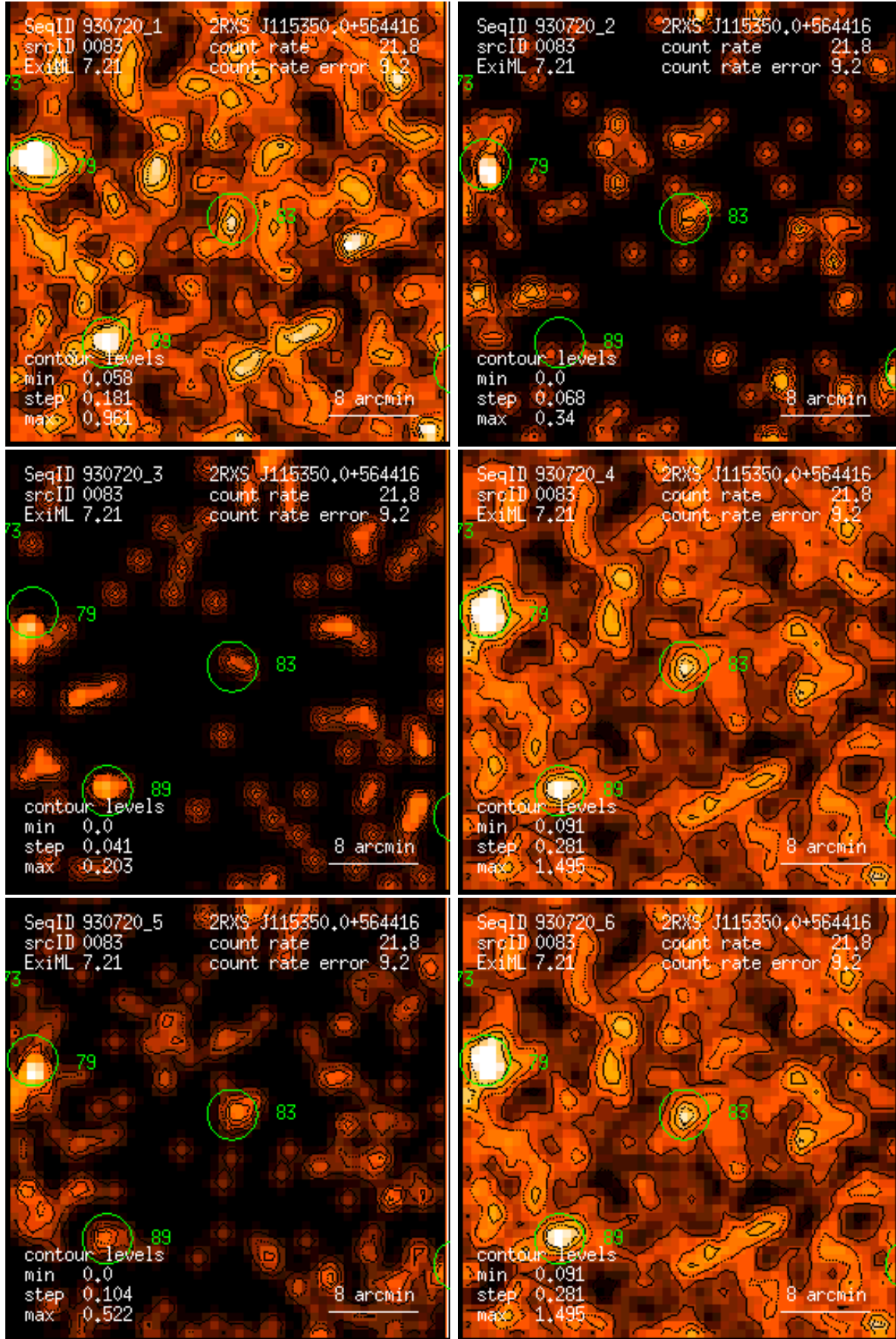
Figure 83: RASS 930720: detection 0083: band rate images, Gaussian filter: (1) PSPC channels 11 – 41, (2) 52 – 90, (3) 91 – 201, (4) 11 – 235, (5) 52 – 201, (6) 11 – 201. Broad band rates in counts/ks. Band rate contour levels in counts/ks/arcmin 2 .
