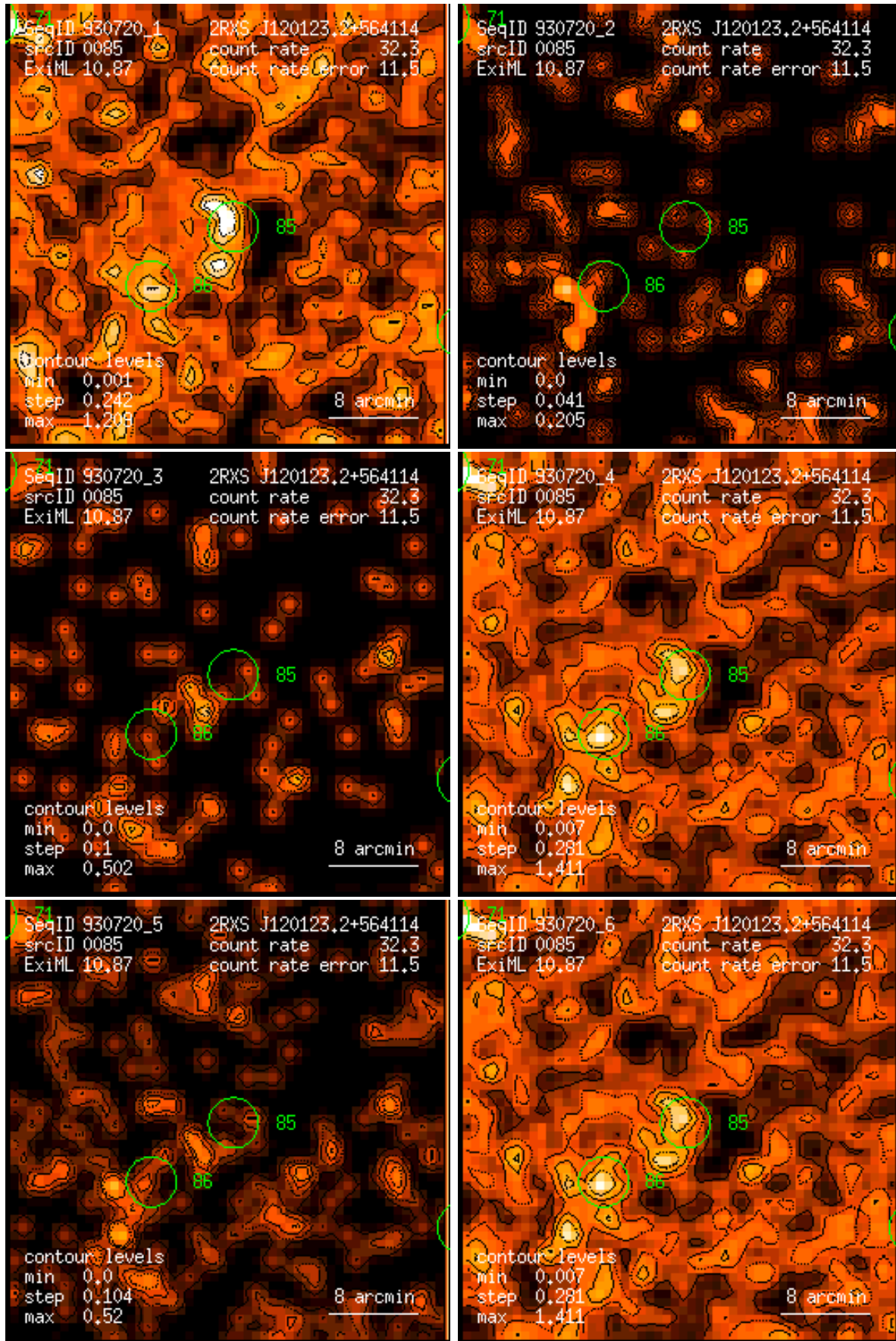
Figure 85: RASS 930720: detection 0085: band rate images, Gaussian filter: (1) PSPC channels 11 – 41, (2) 52 – 90, (3) 91 – 201, (4) 11 – 235, (5) 52 – 201, (6) 11 – 201. Broad band rates in counts/ks. Band rate contour levels in counts/ks/arcmin 2 .
