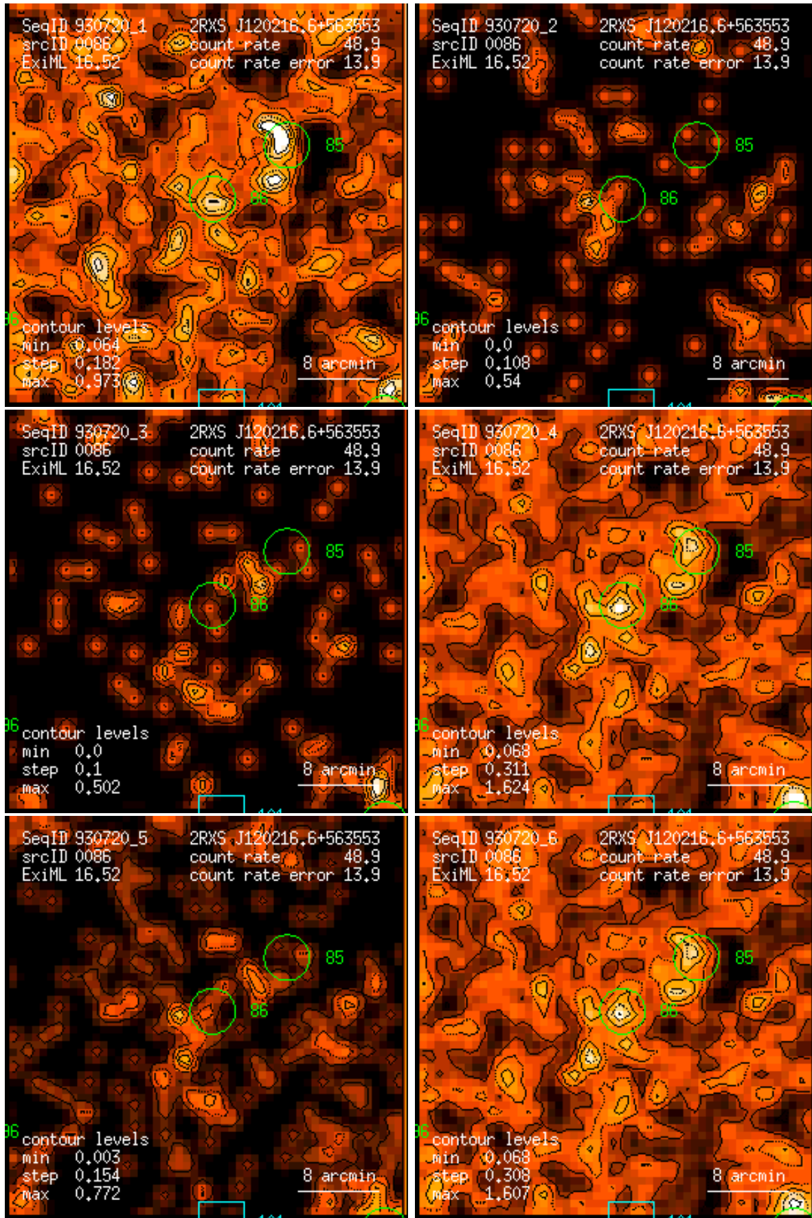
Figure 86: RASS 930720: detection 0086: band rate images, Gaussian filter: (1) PSPC channels 11 – 41, (2) 52 – 90, (3) 91 – 201, (4) 11 – 235, (5) 52 – 201, (6) 11 – 201. Broad band rates in counts/ks. Band rate contour levels in counts/ks/arcmin 2 .
