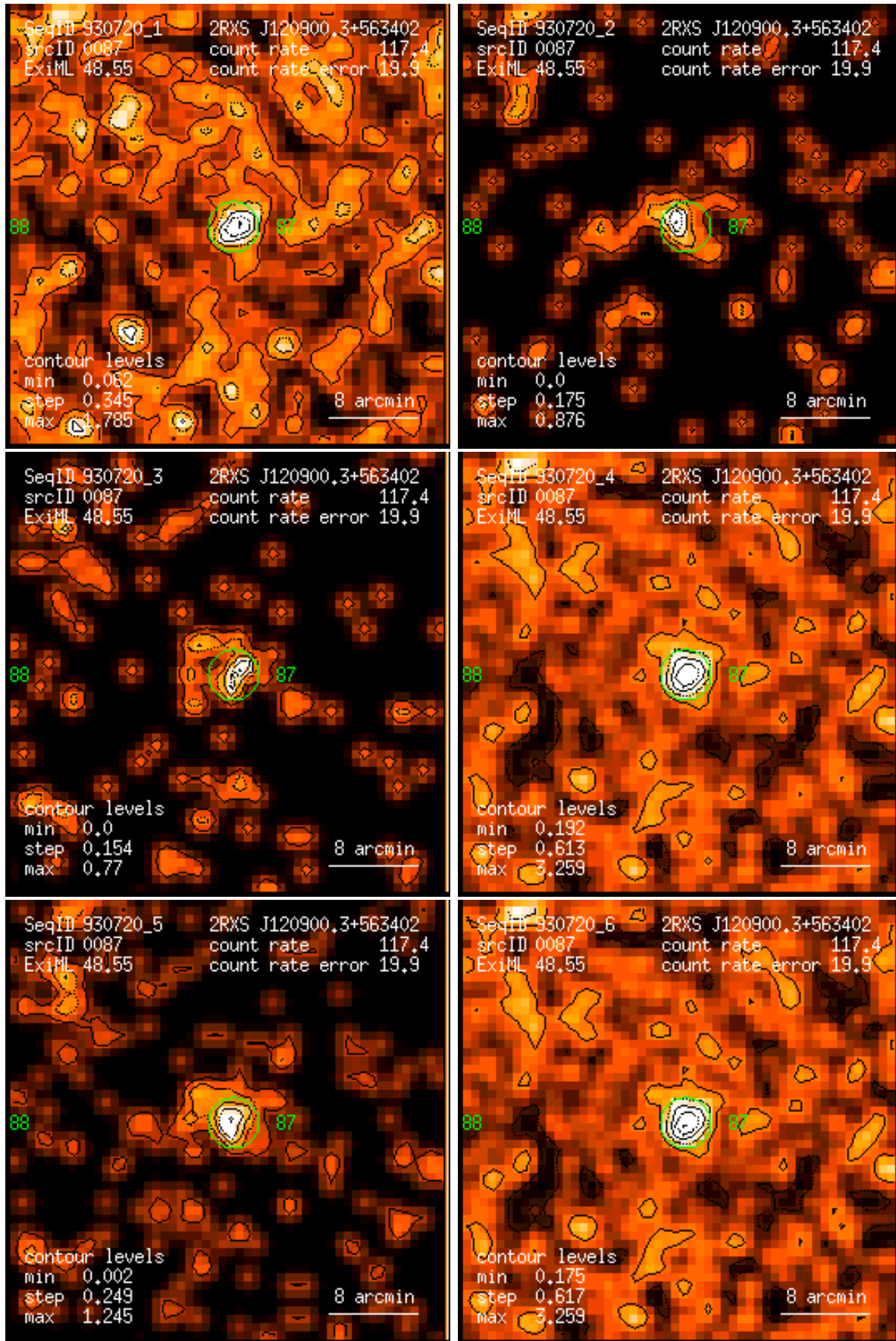
Figure 87: RASS 930720: detection 0087: band rate images, Gaussian filter: (1) PSPC channels 11 – 41, (2) 52 – 90, (3) 91 – 201, (4) 11 – 235, (5) 52 – 201, (6) 11 – 201. Broad band rates in counts/ks. Band rate contour levels in counts/ks/arcmin 2 .
