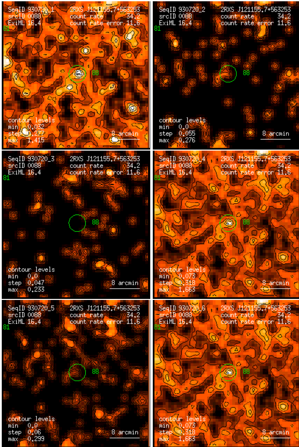
Figure 88: RASS 930720: detection 0088: band rate images, Gaussian filter: (1) PSPC channels 11 – 41, (2) 52 – 90, (3) 91 – 201, (4) 11 – 235, (5) 52 – 201, (6) 11 – 201. Broad band rates in counts/ks. Band rate contour levels in counts/ks/arcmin 2 .
