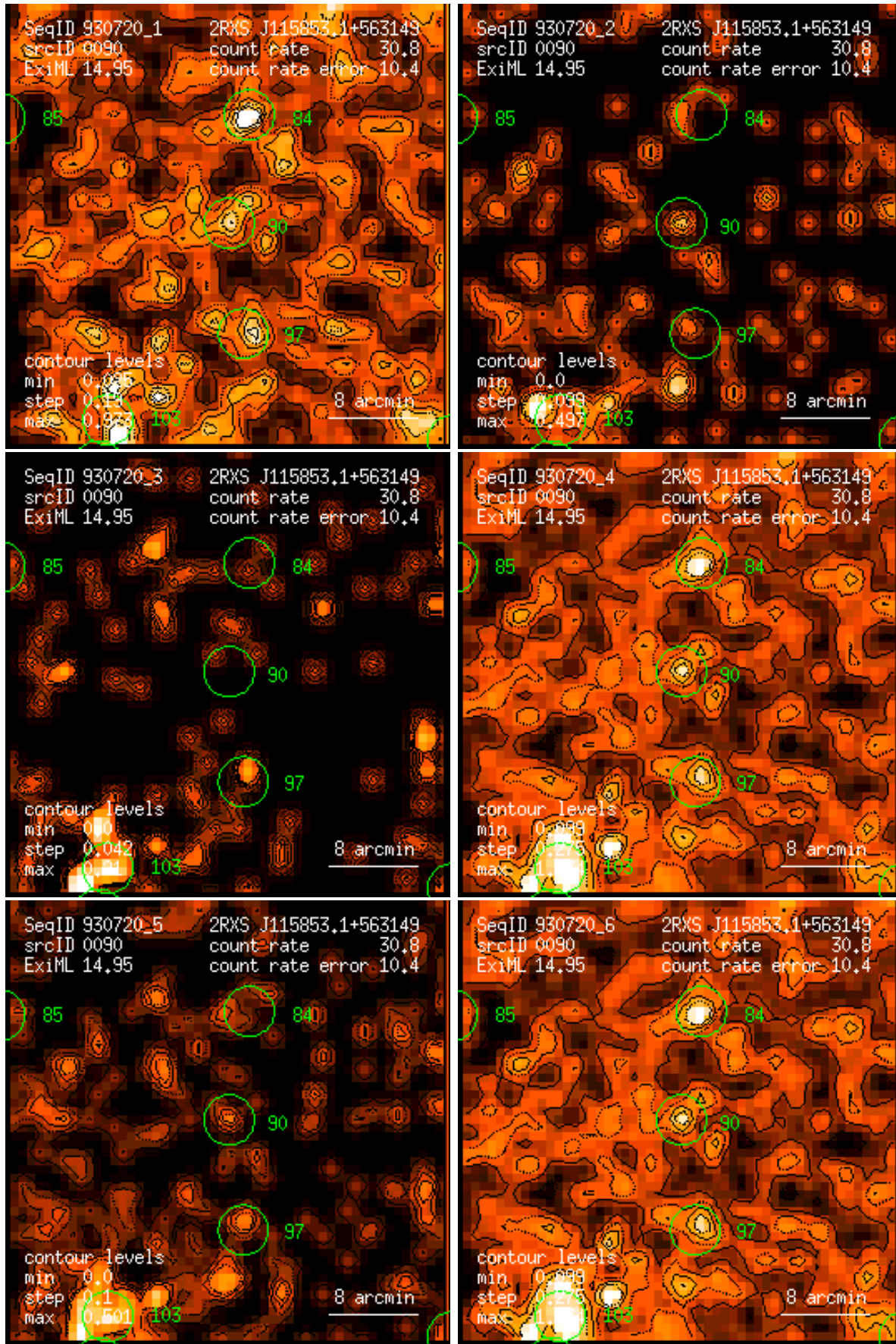
Figure 90: RASS 930720: detection 0090: band rate images, Gaussian filter: (1) PSPC channels 11 – 41, (2) 52 – 90, (3) 91 – 201, (4) 11 – 235, (5) 52 – 201, (6) 11 – 201. Broad band rates in counts/ks. Band rate contour levels in counts/ks/arcmin 2 .
