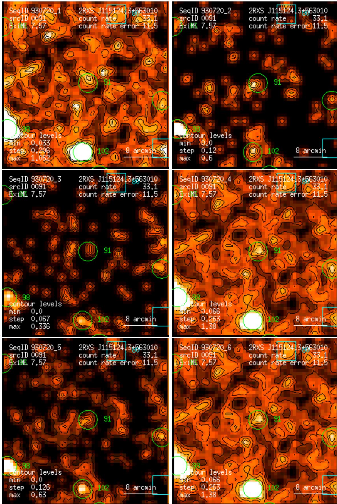
Figure 91: RASS 930720: detection 0091: band rate images, Gaussian filter: (1) PSPC channels 11 – 41, (2) 52 – 90, (3) 91 – 201, (4) 11 – 235, (5) 52 – 201, (6) 11 – 201. Broad band rates in counts/ks. Band rate contour levels in counts/ks/arcmin 2 .
