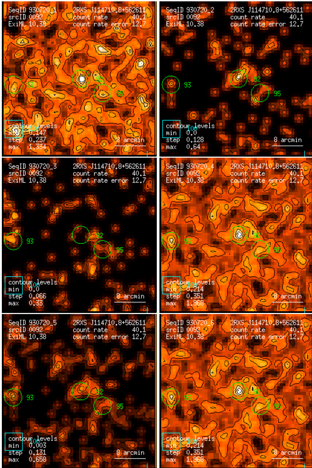
Figure 92: RASS 930720: detection 0092: band rate images, Gaussian filter: (1) PSPC channels 11 – 41, (2) 52 – 90, (3) 91 – 201, (4) 11 – 235, (5) 52 – 201, (6) 11 – 201. Broad band rates in counts/ks. Band rate contour levels in counts/ks/arcmin 2 .
