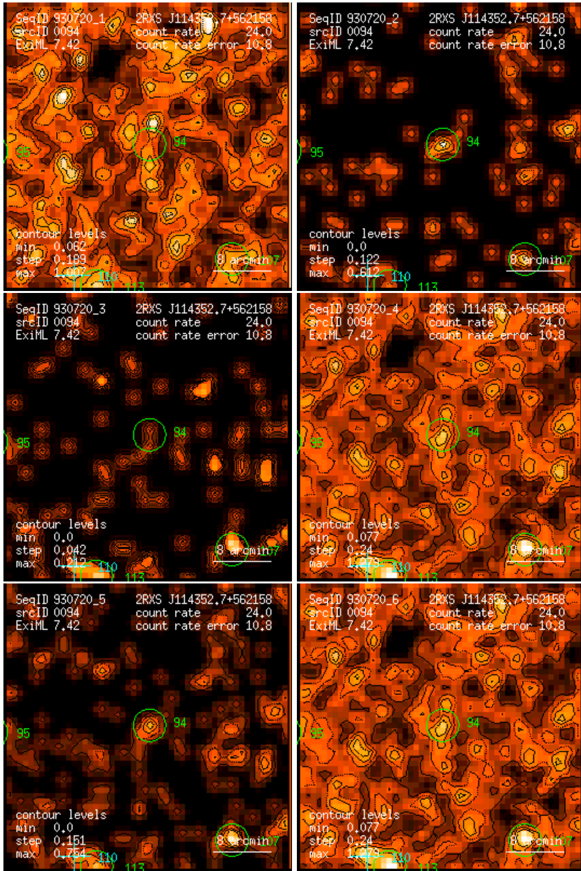
Figure 94: RASS 930720: detection 0094: band rate images, Gaussian filter: (1) PSPC channels 11 – 41, (2) 52 – 90, (3) 91 – 201, (4) 11 – 235, (5) 52 – 201, (6) 11 – 201. Broad band rates in counts/ks. Band rate contour levels in counts/ks/arcmin 2 .
