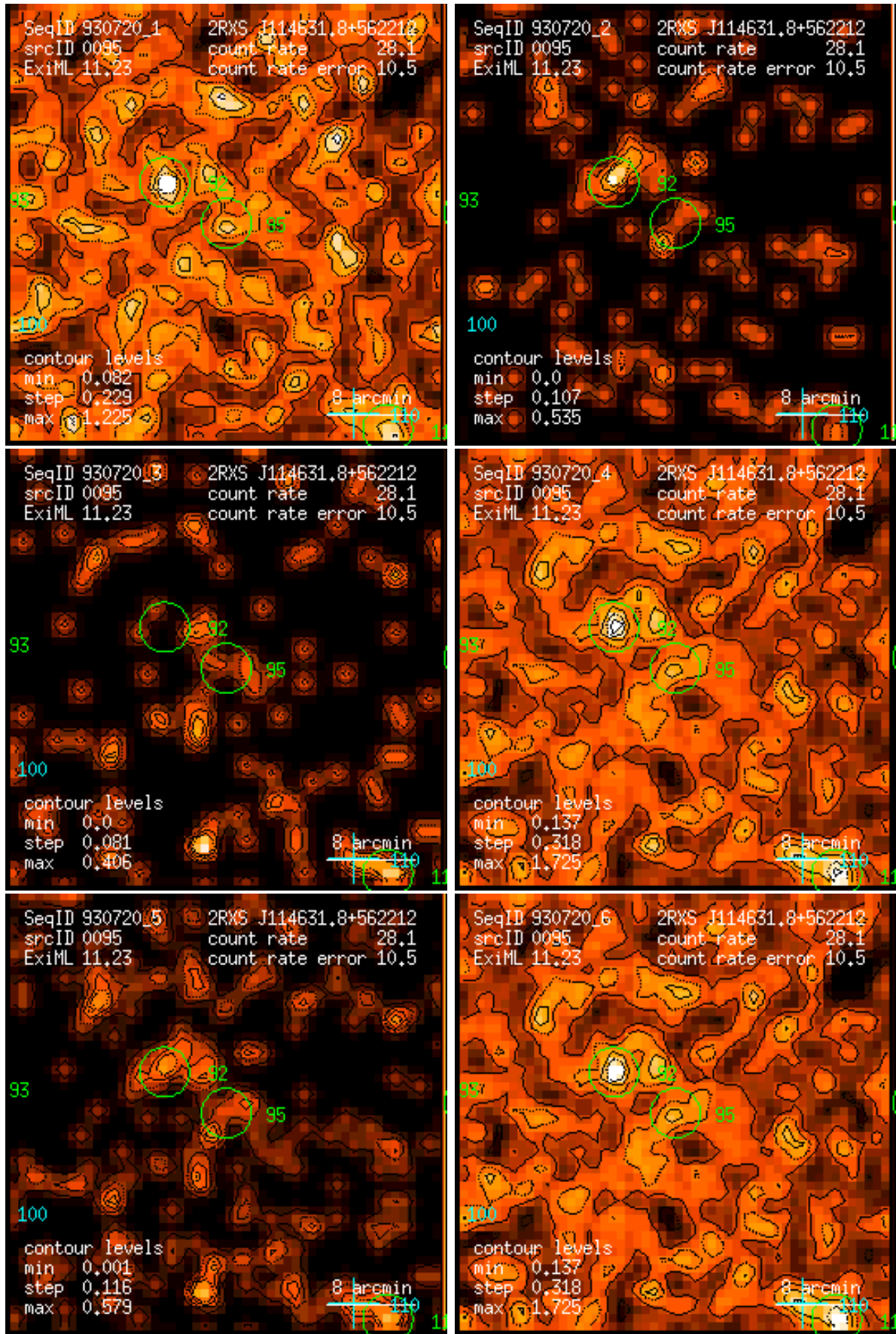
Figure 95: RASS 930720: detection 0095: band rate images, Gaussian filter: (1) PSPC channels 11 – 41, (2) 52 – 90, (3) 91 – 201, (4) 11 – 235, (5) 52 – 201, (6) 11 – 201. Broad band rates in counts/ks. Band rate contour levels in counts/ks/arcmin 2 .
