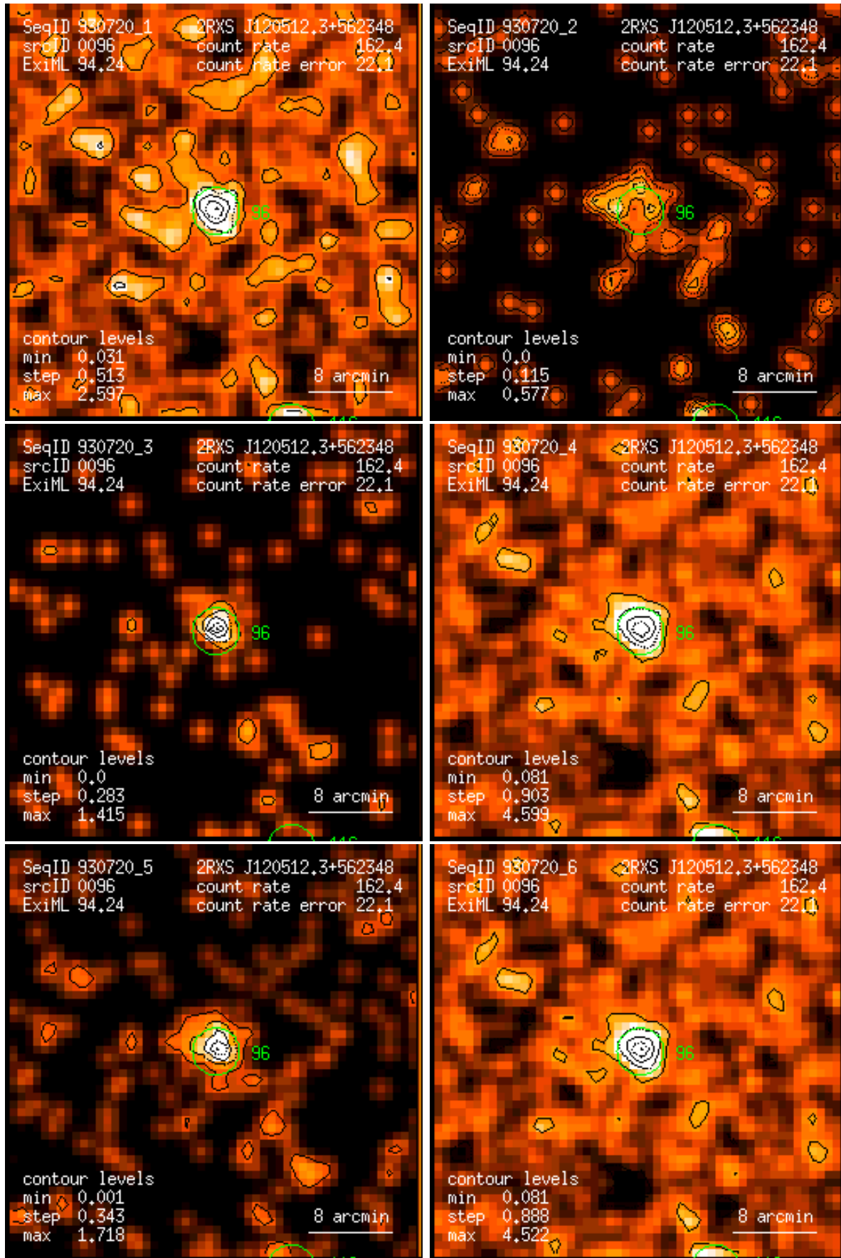
Figure 96: RASS 930720: detection 0096: band rate images, Gaussian filter: (1) PSPC channels 11 – 41, (2) 52 – 90, (3) 91 – 201, (4) 11 – 235, (5) 52 – 201, (6) 11 – 201. Broad band rates in counts/ks. Band rate contour levels in counts/ks/arcmin 2 .
