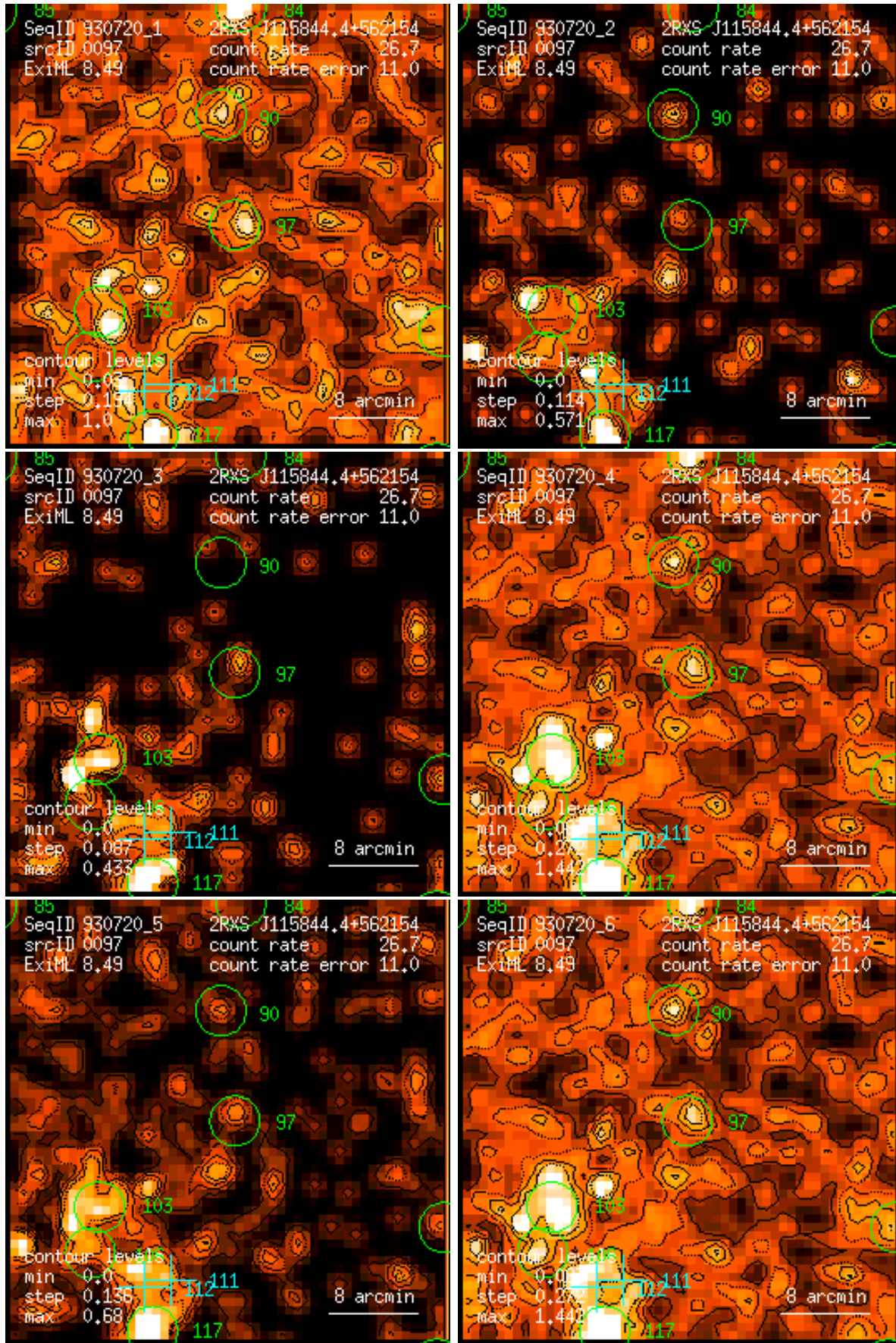
Figure 97: RASS 930720: detection 0097: band rate images, Gaussian filter: (1) PSPC channels 11 – 41, (2) 52 – 90, (3) 91 – 201, (4) 11 – 235, (5) 52 – 201, (6) 11 – 201. Broad band rates in counts/ks. Band rate contour levels in counts/ks/arcmin 2 .
