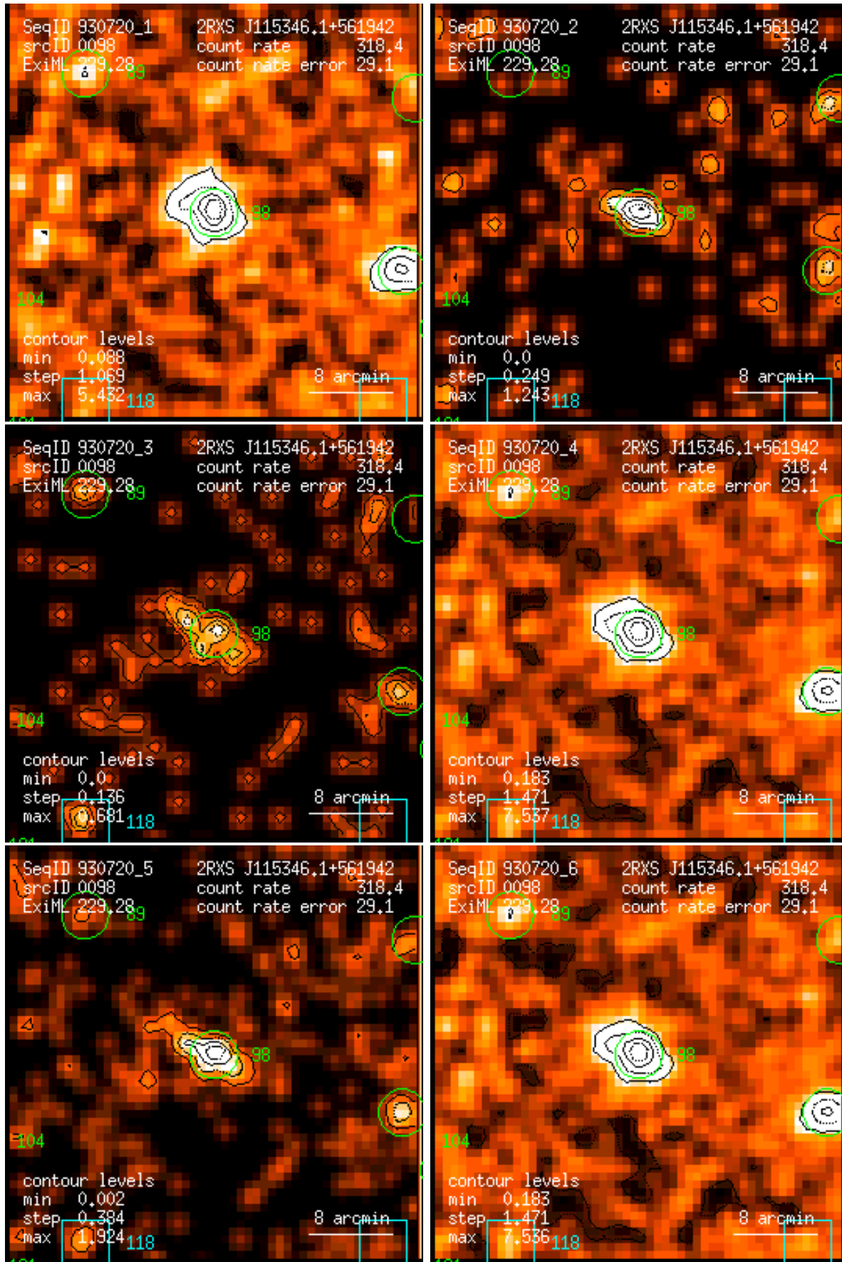
Figure 98: RASS 930720: detection 0098: band rate images, Gaussian filter: (1) PSPC channels 11 – 41, (2) 52 – 90, (3) 91 – 201, (4) 11 – 235, (5) 52 – 201, (6) 11 – 201. Broad band rates in counts/ks. Band rate contour levels in counts/ks/arcmin 2 .
