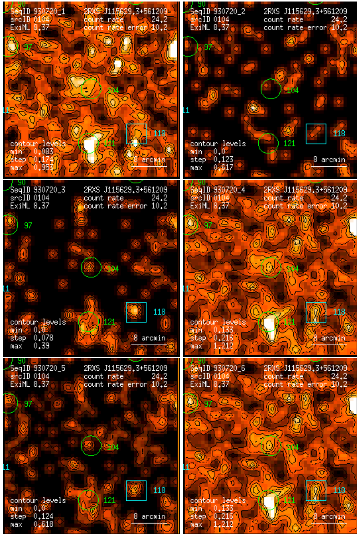
Figure 104: RASS 930720: detection 0104: band rate images, Gaussian filter: (1) PSPC channels 11 – 41, (2) 52 – 90, (3) 91 – 201, (4) 11 – 235, (5) 52 – 201, (6) 11 – 201. Broad band rates in counts/ks. Band rate contour levels in counts/ks/arcmin 2 .
