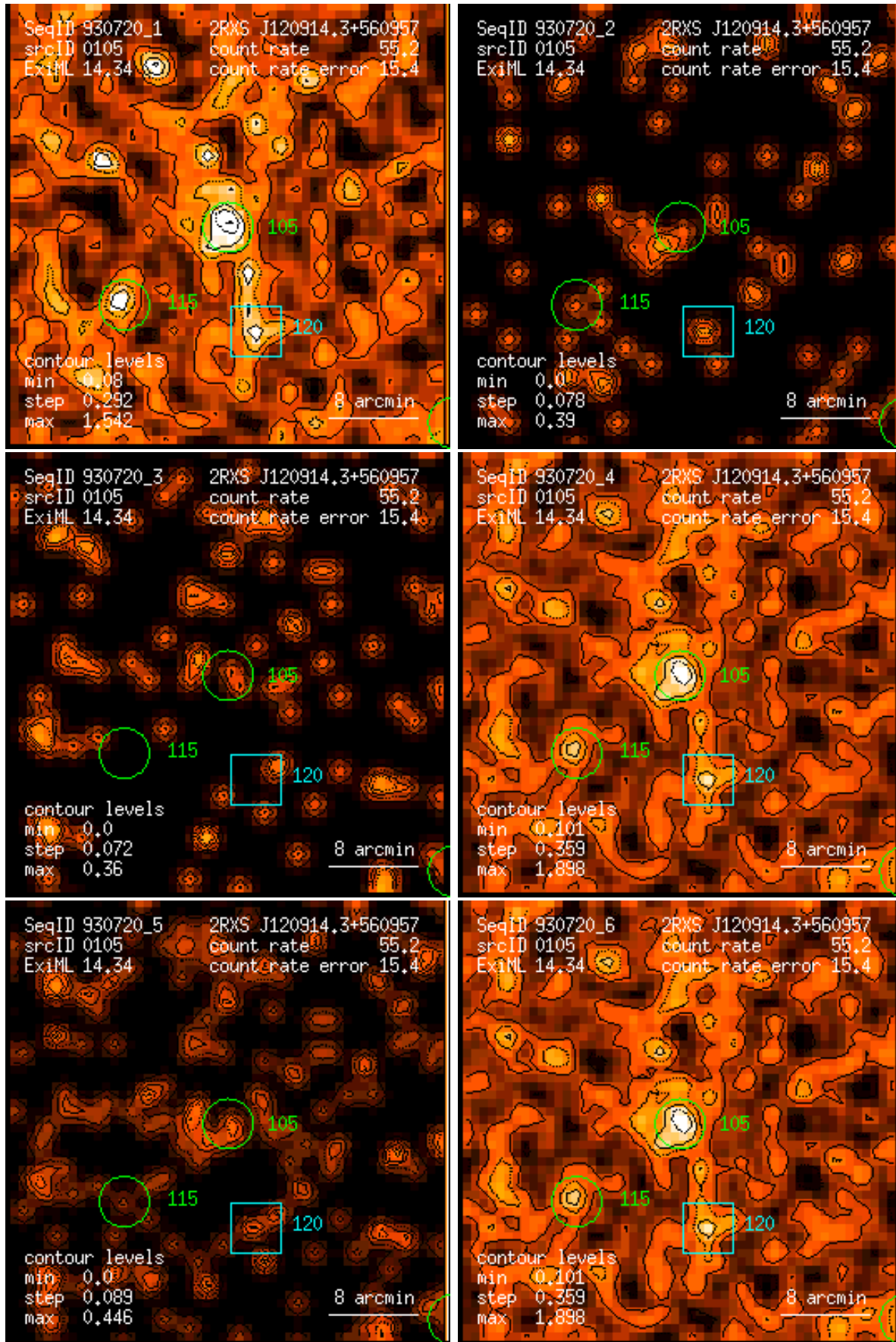
Figure 105: RASS 930720: detection 0105: band rate images, Gaussian filter: (1) PSPC channels 11 – 41, (2) 52 – 90, (3) 91 – 201, (4) 11 – 235, (5) 52 – 201, (6) 11 – 201. Broad band rates in counts/ks. Band rate contour levels in counts/ks/arcmin 2 .
