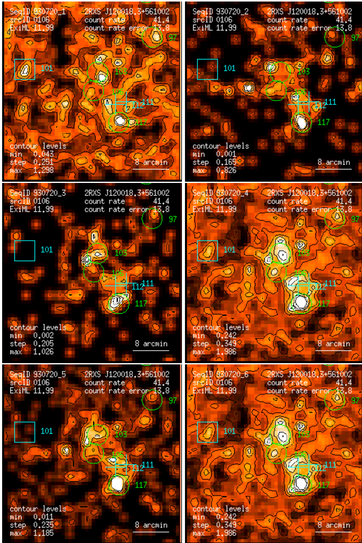
Figure 106: RASS 930720: detection 0106: band rate images, Gaussian filter: (1) PSPC channels 11 – 41, (2) 52 – 90, (3) 91 – 201, (4) 11 – 235, (5) 52 – 201, (6) 11 – 201. Broad band rates in counts/ks. Band rate contour levels in counts/ks/arcmin 2 .
