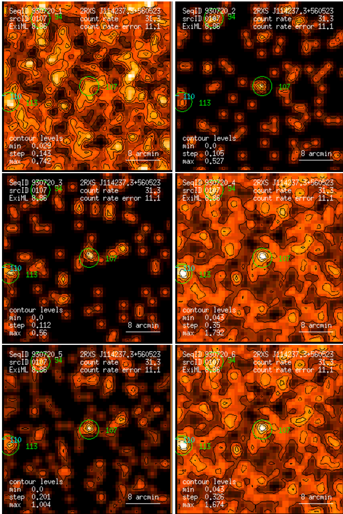
Figure 107: RASS 930720: detection 0107: band rate images, Gaussian filter: (1) PSPC channels 11 – 41, (2) 52 – 90, (3) 91 – 201, (4) 11 – 235, (5) 52 – 201, (6) 11 – 201. Broad band rates in counts/ks. Band rate contour levels in counts/ks/arcmin 2 .
