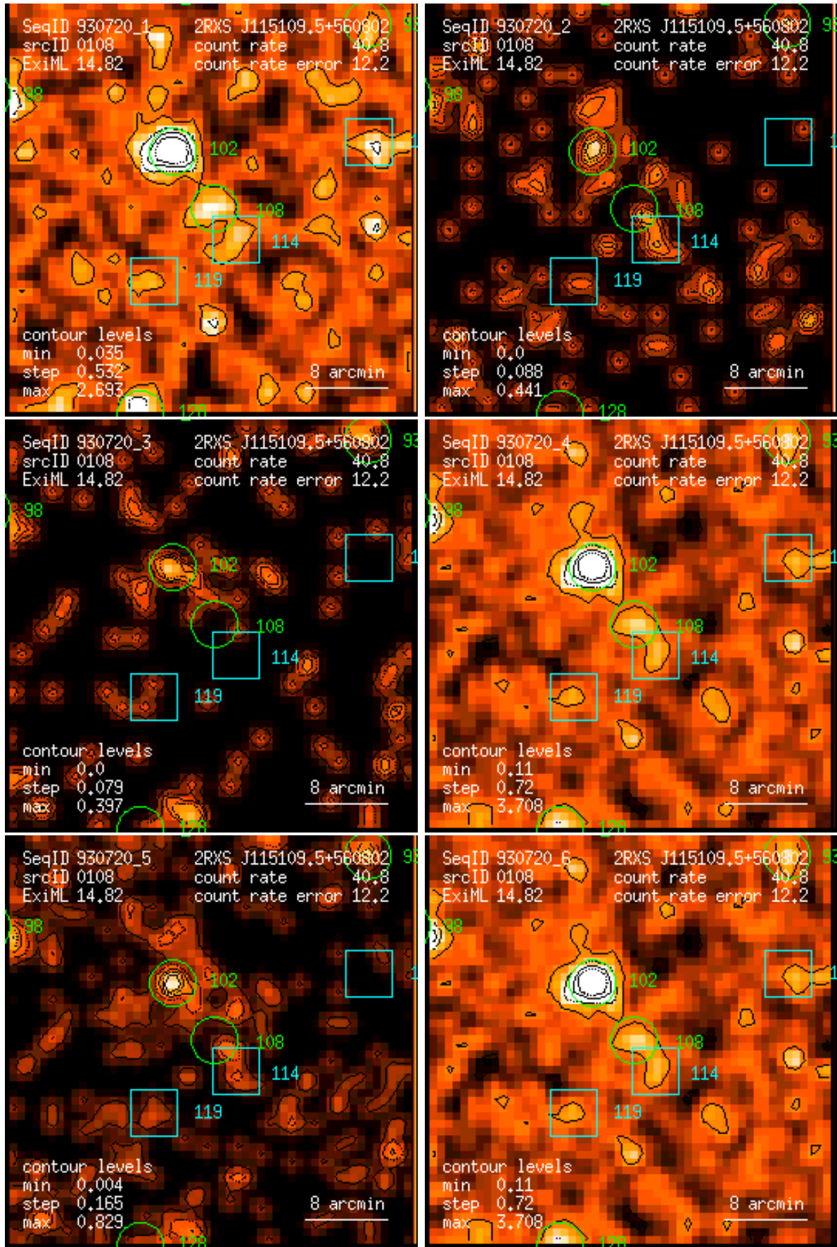
Figure 108: RASS 930720: detection 0108: band rate images, Gaussian filter: (1) PSPC channels 11 – 41, (2) 52 – 90, (3) 91 – 201, (4) 11 – 235, (5) 52 – 201, (6) 11 – 201. Broad band rates in counts/ks. Band rate contour levels in counts/ks/arcmin 2 .
