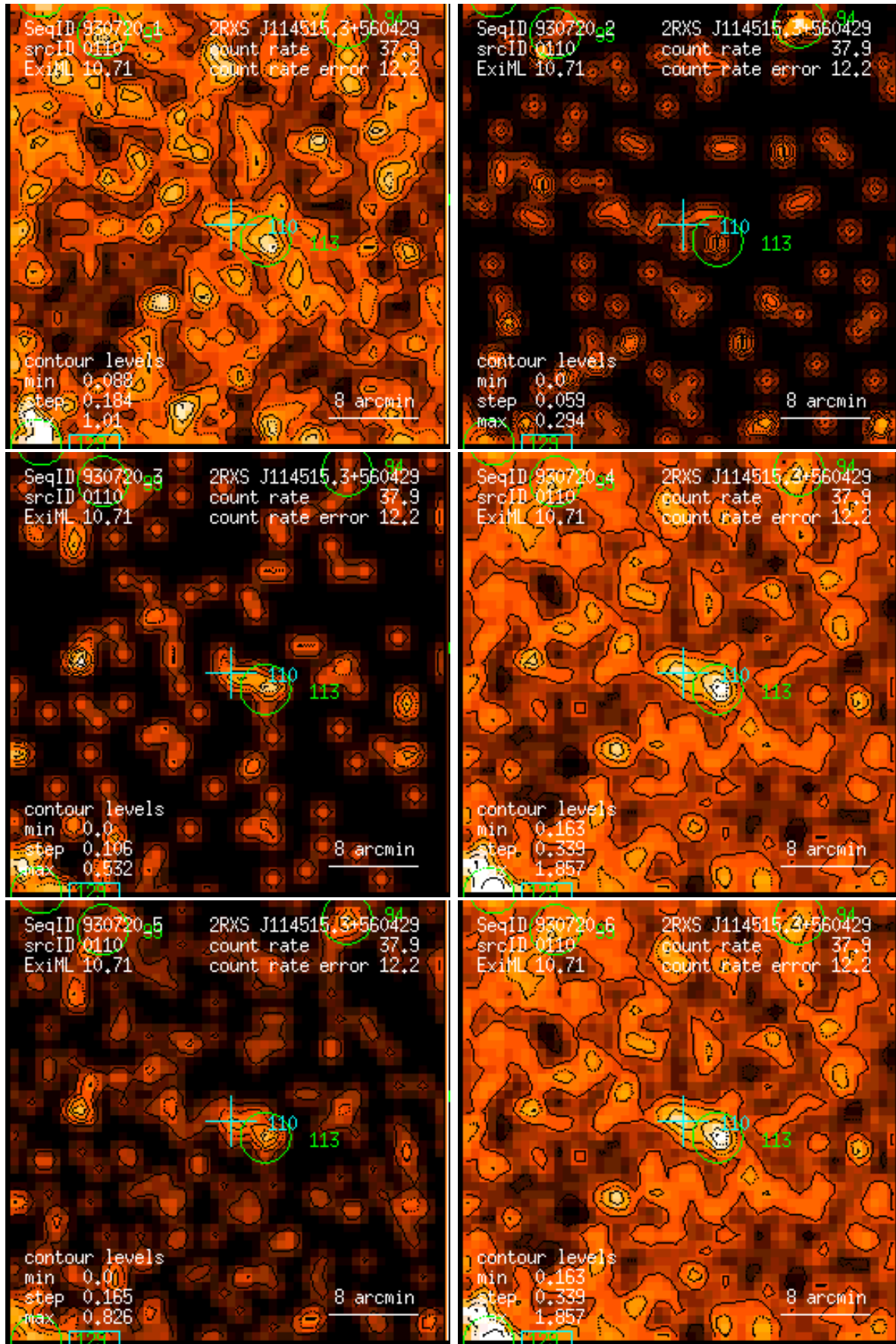
Figure 110: RASS 930720: detection 0110: band rate images, Gaussian filter: (1) PSPC channels 11 – 41, (2) 52 – 90, (3) 91 – 201, (4) 11 – 235, (5) 52 – 201, (6) 11 – 201. Broad band rates in counts/ks. Band rate contour levels in counts/ks/arcmin 2 .
