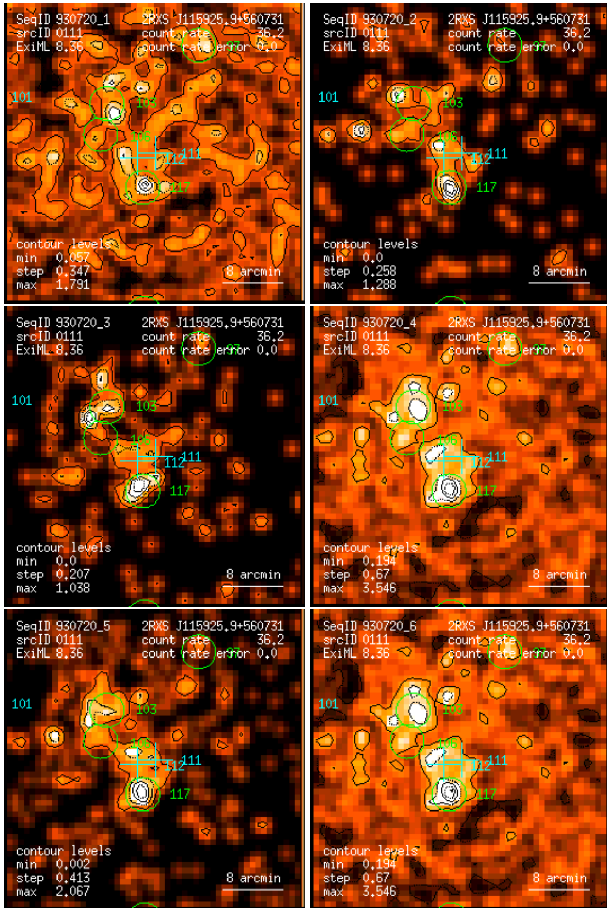
Figure 111: RASS 930720: detection 0111: band rate images, Gaussian filter: (1) PSPC channels 11 – 41, (2) 52 – 90, (3) 91 – 201, (4) 11 – 235, (5) 52 – 201, (6) 11 – 201. Broad band rates in counts/ks. Band rate contour levels in counts/ks/arcmin 2 .
