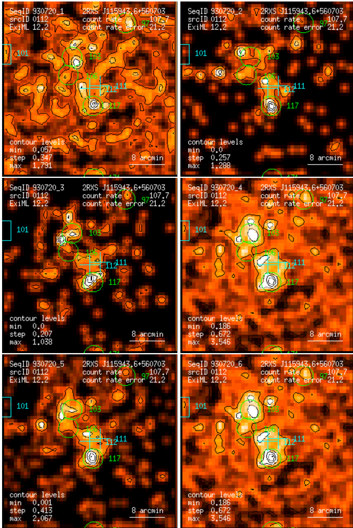
Figure 112: RASS 930720: detection 0112: band rate images, Gaussian filter: (1) PSPC channels 11 – 41, (2) 52 – 90, (3) 91 – 201, (4) 11 – 235, (5) 52 – 201, (6) 11 – 201. Broad band rates in counts/ks. Band rate contour levels in counts/ks/arcmin 2 .
