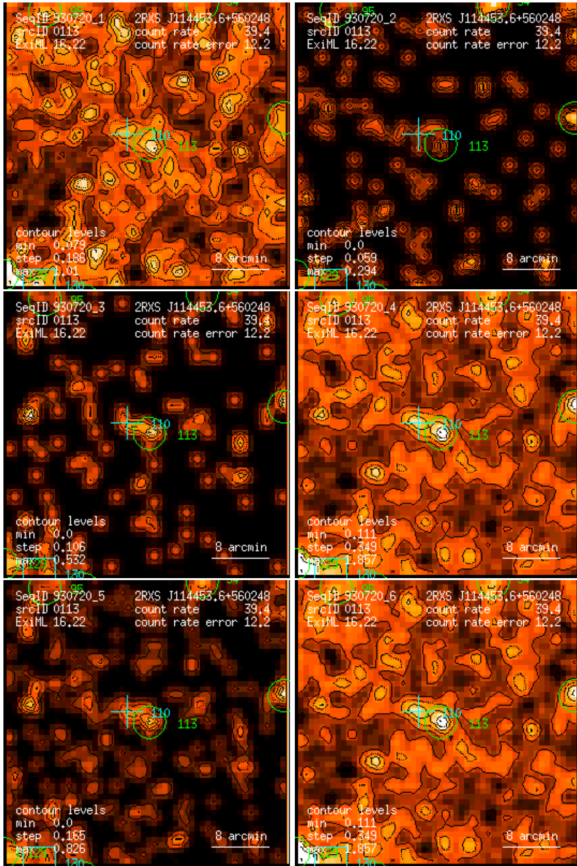
Figure 113: RASS 930720: detection 0113: band rate images, Gaussian filter: (1) PSPC channels 11 – 41, (2) 52 – 90, (3) 91 – 201, (4) 11 – 235, (5) 52 – 201, (6) 11 – 201. Broad band rates in counts/ks. Band rate contour levels in counts/ks/arcmin 2 .
