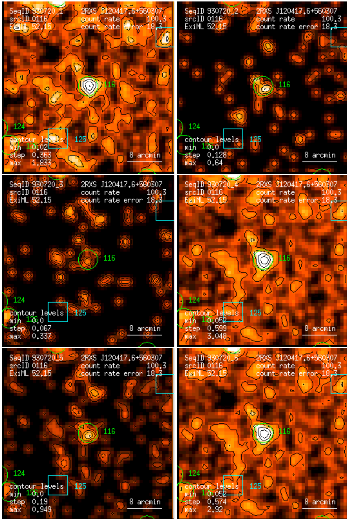
Figure 116: RASS 930720: detection 0116: band rate images, Gaussian filter: (1) PSPC channels 11 – 41, (2) 52 – 90, (3) 91 – 201, (4) 11 – 235, (5) 52 – 201, (6) 11 – 201. Broad band rates in counts/ks. Band rate contour levels in counts/ks/arcmin 2 .
