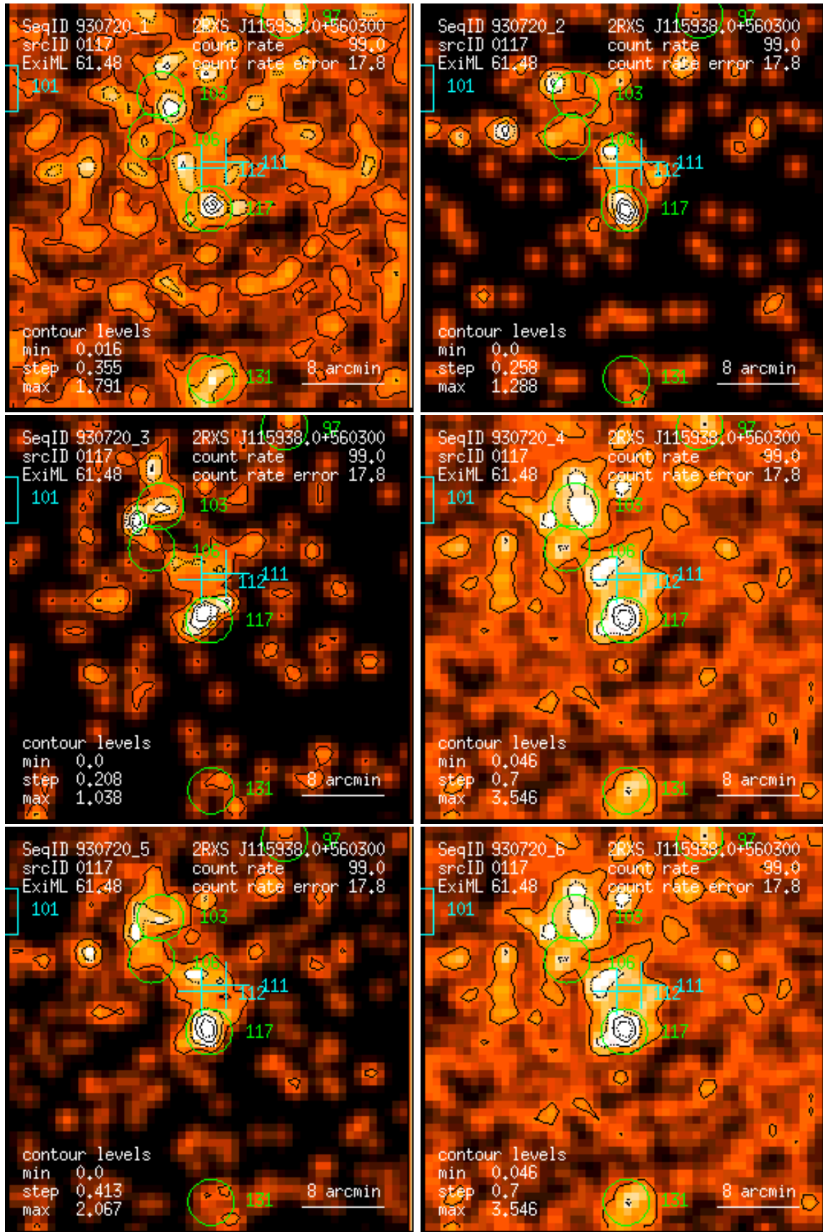
Figure 117: RASS 930720: detection 0117: band rate images, Gaussian filter: (1) PSPC channels 11 – 41, (2) 52 – 90, (3) 91 – 201, (4) 11 – 235, (5) 52 – 201, (6) 11 – 201. Broad band rates in counts/ks. Band rate contour levels in counts/ks/arcmin 2 .
