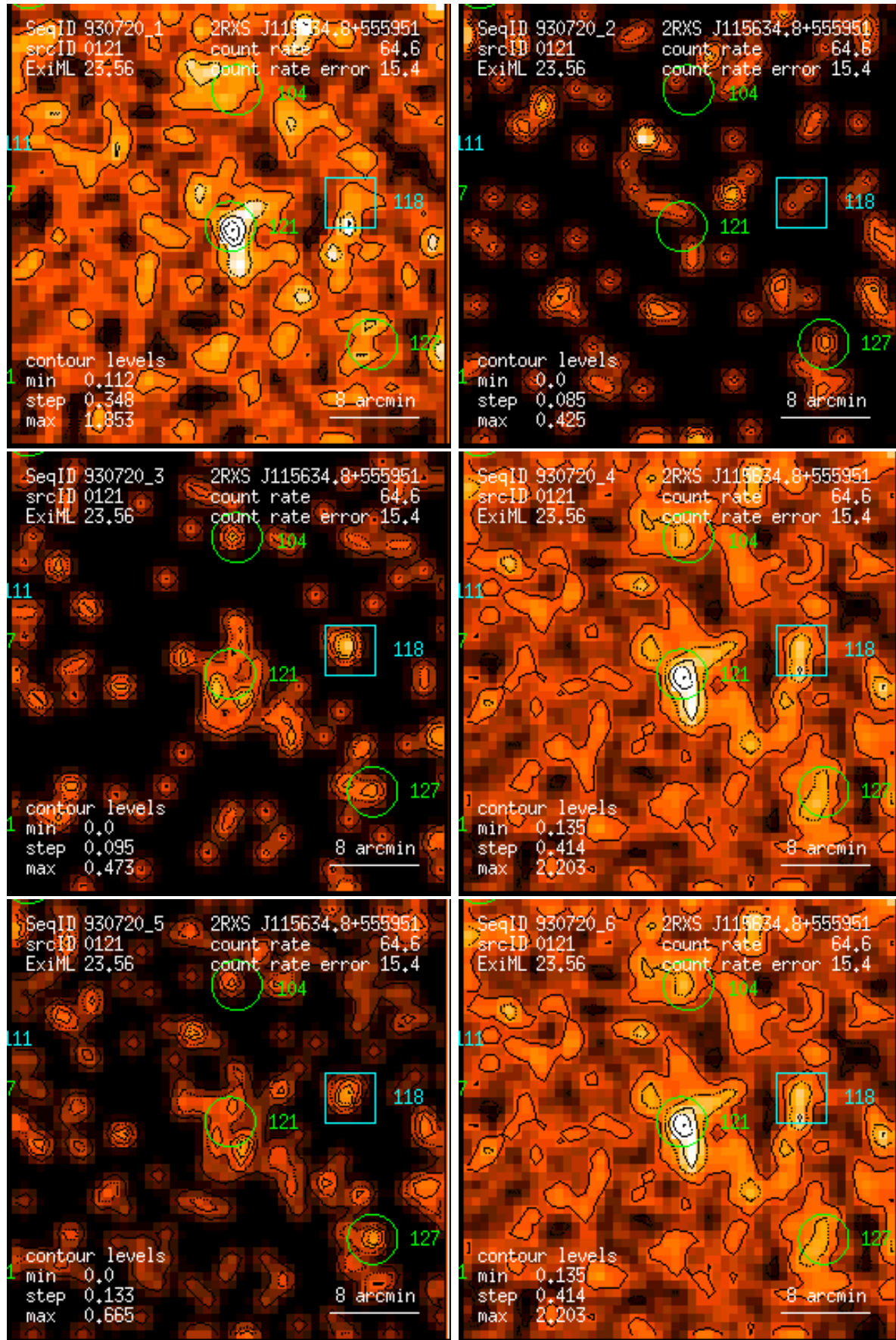
Figure 121: RASS 930720: detection 0121: band rate images, Gaussian filter: (1) PSPC channels 11 – 41, (2) 52 – 90, (3) 91 – 201, (4) 11 – 235, (5) 52 – 201, (6) 11 – 201. Broad band rates in counts/ks. Band rate contour levels in counts/ks/arcmin 2 .
