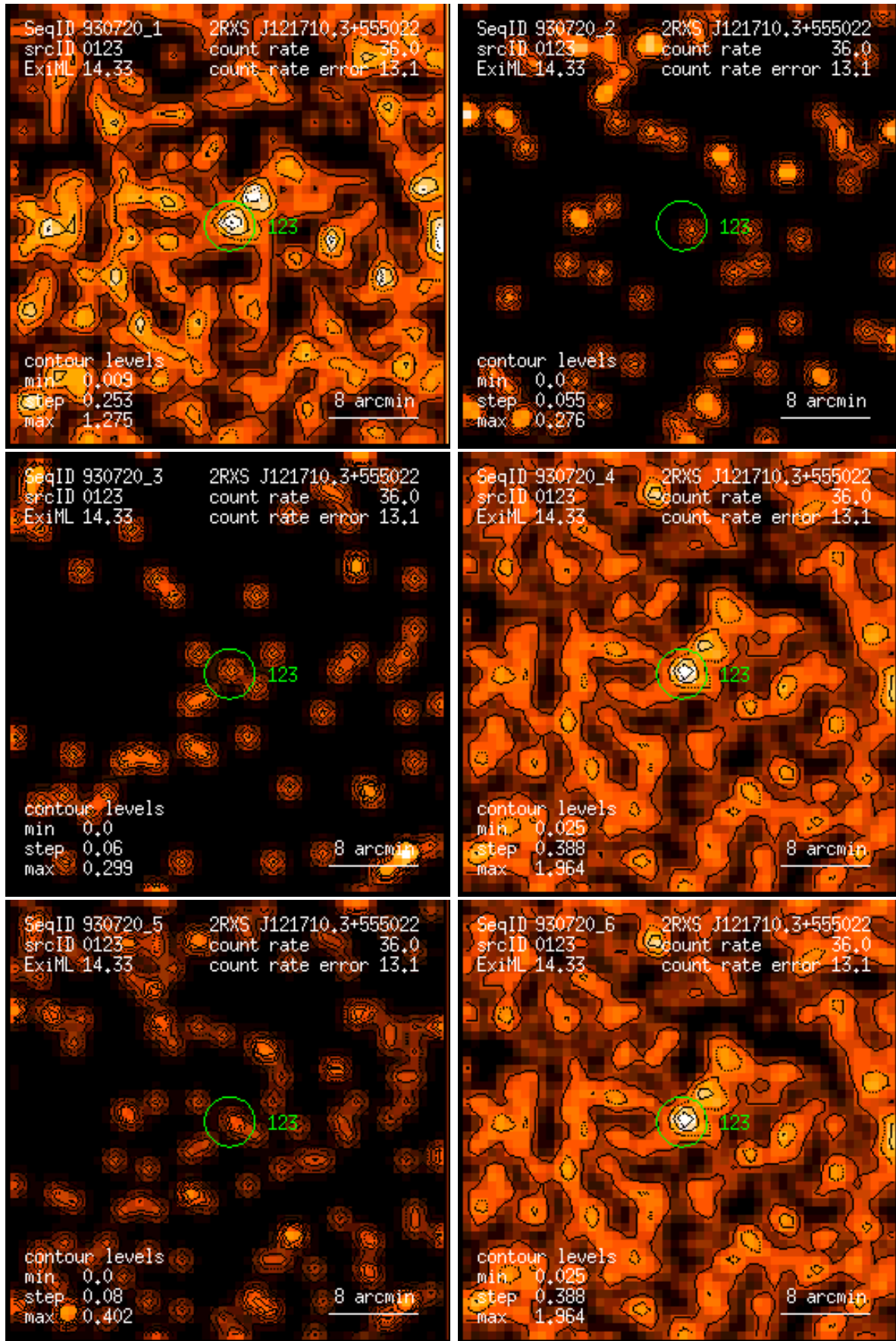
Figure 123: RASS 930720: detection 0123: band rate images, Gaussian filter: (1) PSPC channels 11 – 41, (2) 52 – 90, (3) 91 – 201, (4) 11 – 235, (5) 52 – 201, (6) 11 – 201. Broad band rates in counts/ks. Band rate contour levels in counts/ks/arcmin 2 .
