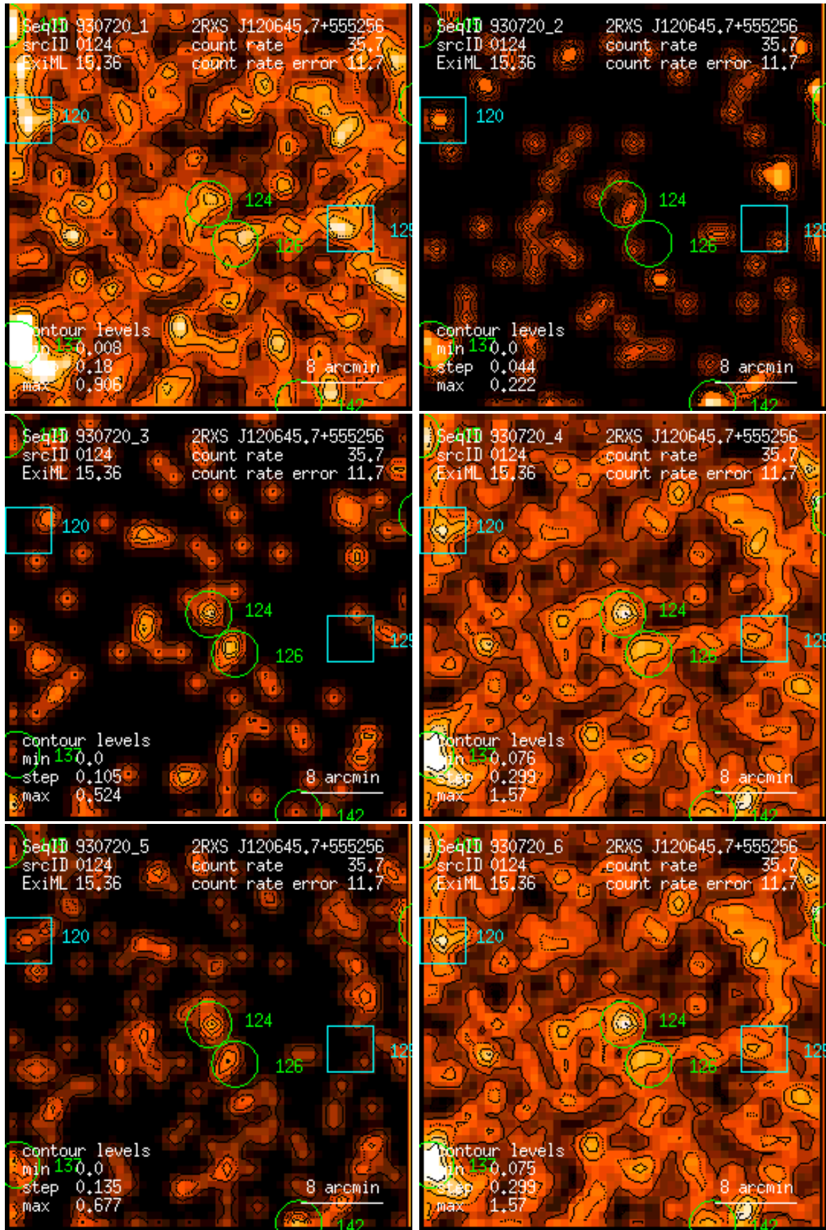
Figure 124: RASS 930720: detection 0124: band rate images, Gaussian filter: (1) PSPC channels 11 – 41, (2) 52 – 90, (3) 91 – 201, (4) 11 – 235, (5) 52 – 201, (6) 11 – 201. Broad band rates in counts/ks. Band rate contour levels in counts/ks/arcmin 2 .
