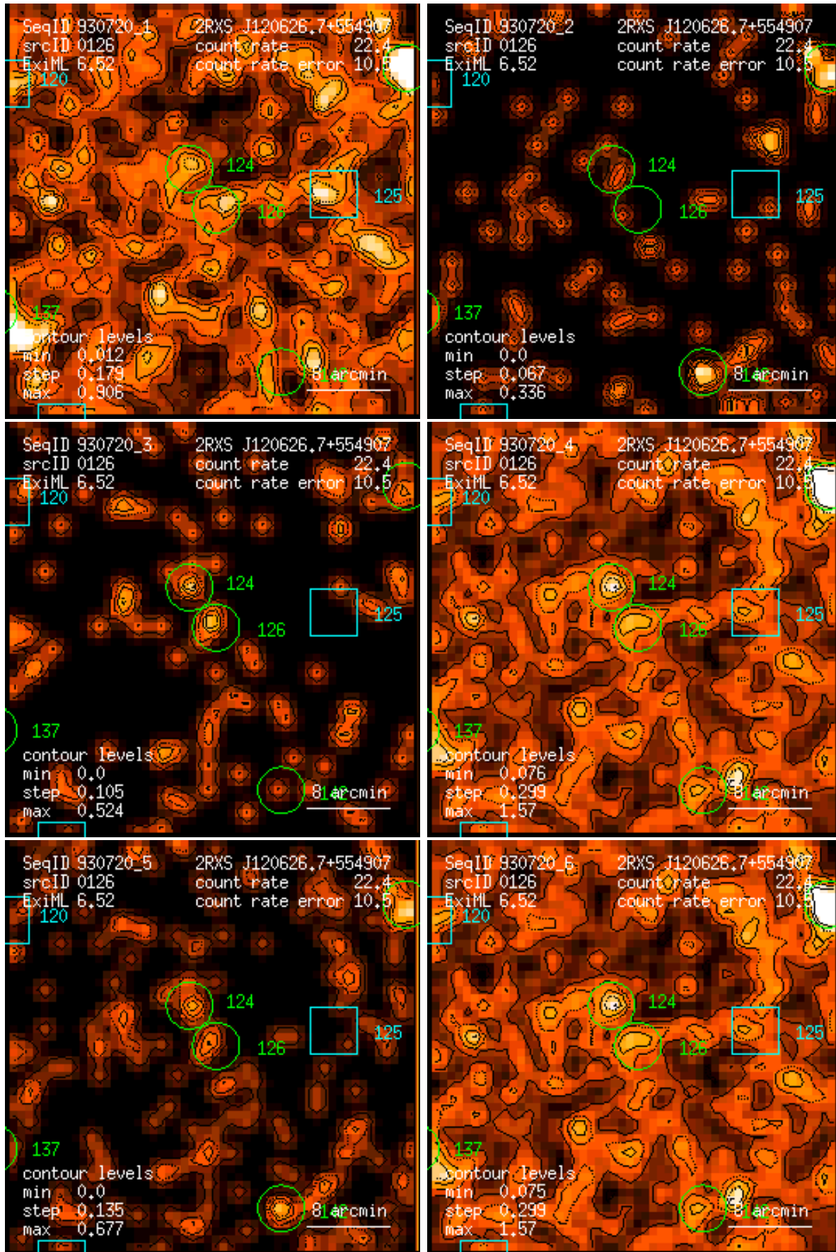
Figure 126: RASS 930720: detection 0126: band rate images, Gaussian filter: (1) PSPC channels 11 – 41, (2) 52 – 90, (3) 91 – 201, (4) 11 – 235, (5) 52 – 201, (6) 11 – 201. Broad band rates in counts/ks. Band rate contour levels in counts/ks/arcmin 2 .
